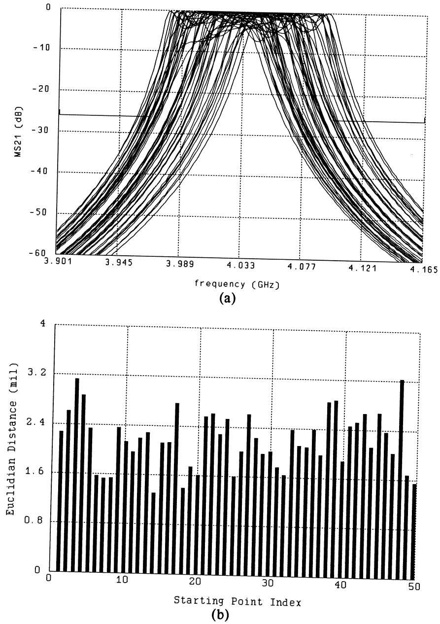
Fig. 6. (a) The empirical model |S_{21}| responses at 50 random starting points and (b) the Euclidian distances between the perturbed starting points and the reference minimax solution.
