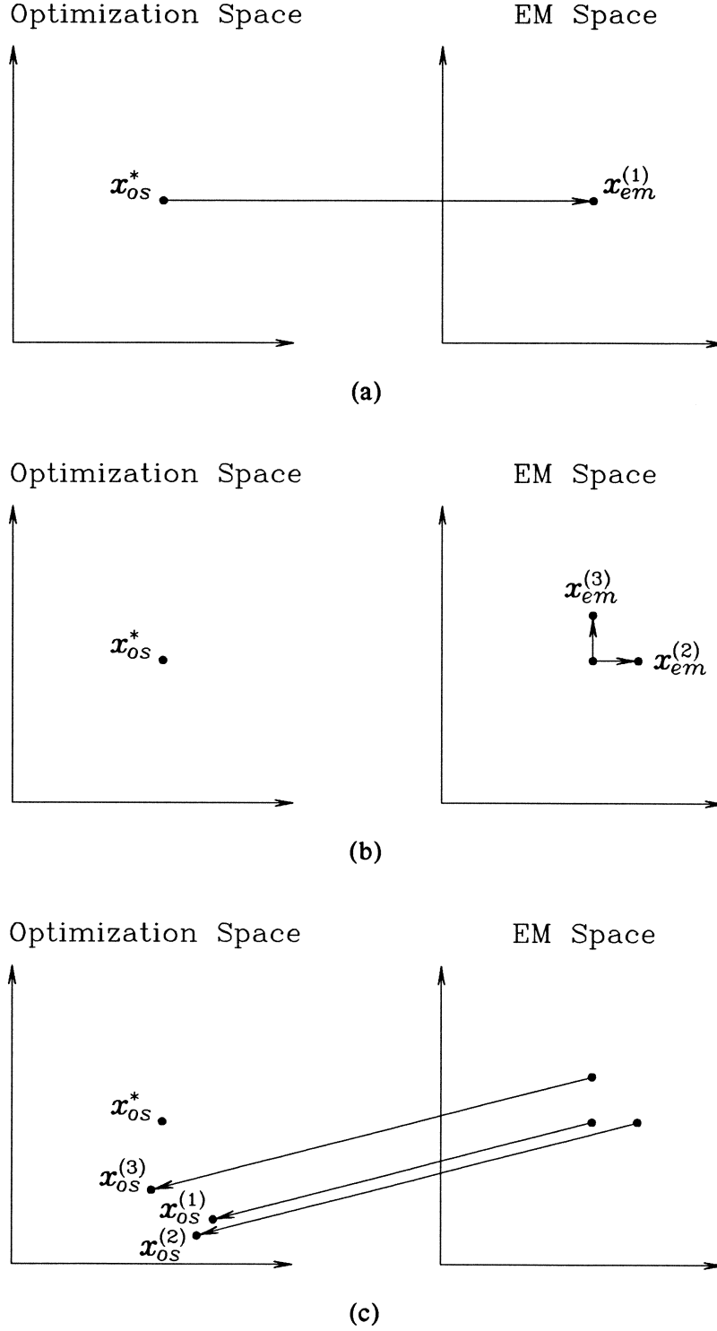
Fig. 2. Illustration of the original SM algorithm: (a) set x_{em}^{(1)} = x_{os}^* , (b) generate, at least, m - 1 additional base points around x_{em}^{(1)} , (c) perform X_{os} -space model parameter extraction according to (6).
