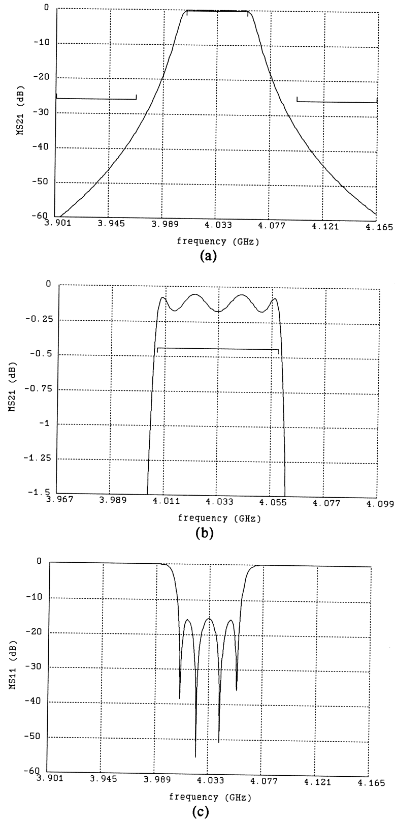
Fig. 5. The OSA90/hope empirical model responses after minimax optimization. The |S_{21}| response for (a) the overall band and (b) the passband details. (c) The |S_{11}| response of the filter.
