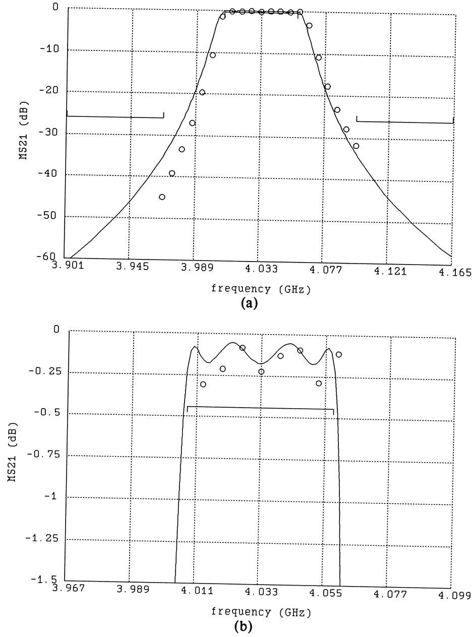
Fig. 16. The em simulated |S_{21}| response of the HTS filter at the solution obtained using the quasi-Newton SM optimization method ( \circ ). The OSA90/hope empirical model solution (—) is shown for comparison. Responses for (a) the overall band and (b) the passband in more detail.
