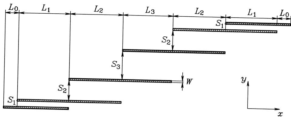
Fig. 4. The structure of the HTS filter [3, 5].
