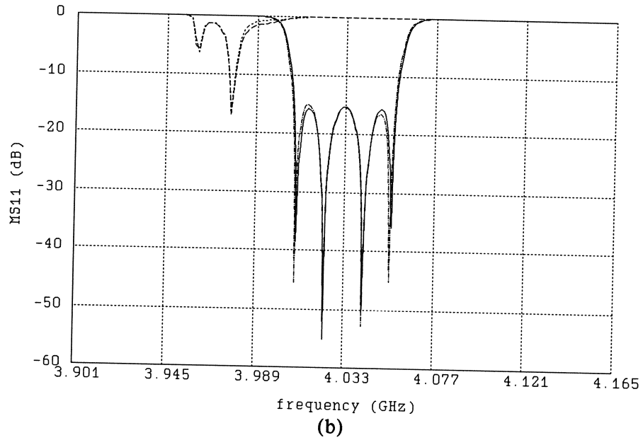
Fig. 9. A comparison between the (a) |S_{21}| and (b) |S_{11}| empirical model and corresponding em responses at the two minimax solutions.
