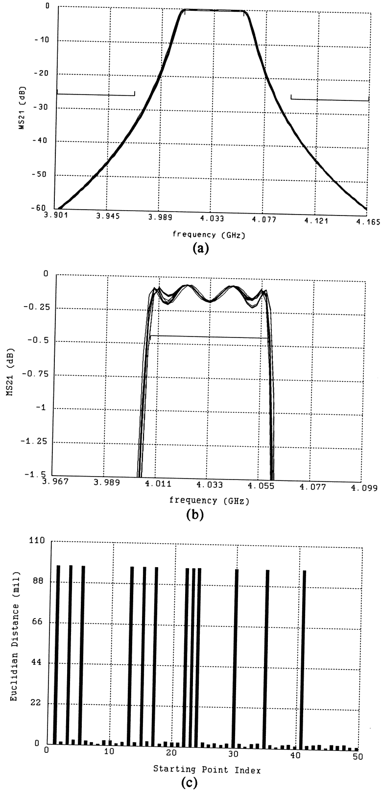
Fig. 7. The empirical model |S_{21}| responses at the 50 optimized solutions for (a) the overall band, (b) the passband in more detail and (c) the Euclidian distances between the optimized and reference minimax solution.
