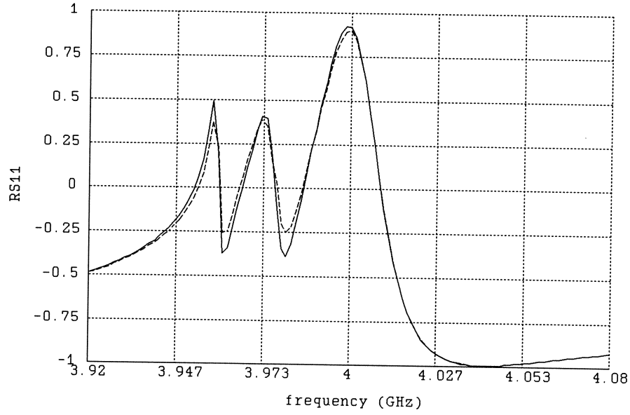
Fig. 14. \text{Re}\{S_{11}\} simulated using the empirical model (—) and em (---) after Phase 2 of the FSM algorithm.
