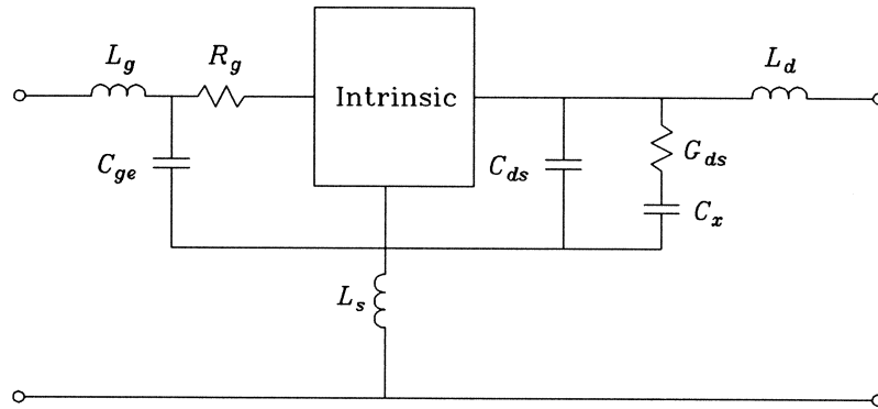
Fig. 12. Equivalent circuit for the SPICE MESFET model.
