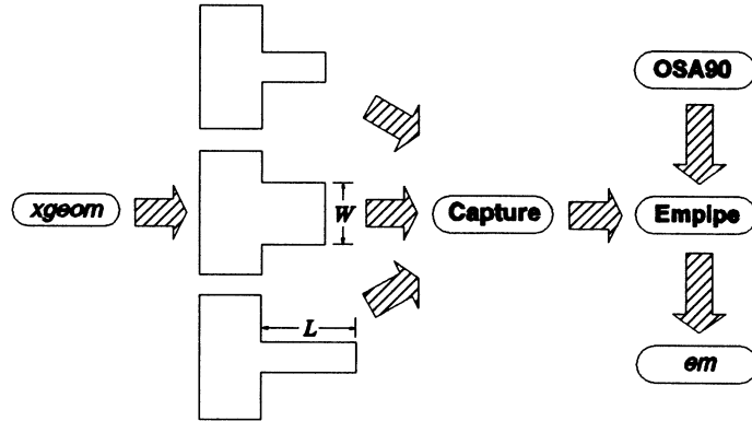
Fig. 3. Illustration of Geometry Capture for parameterizing the step structure w.r.t. L and W .
