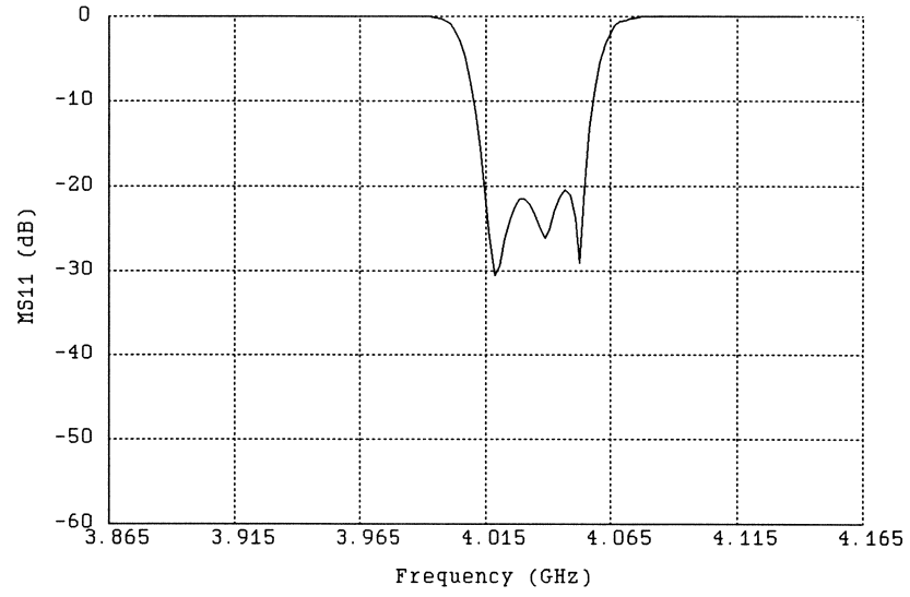
Fig. 11. The em simulated |S_{11}| response of the HTS parallel coupled-line filter at the solution obtained using the SM optimization method.
