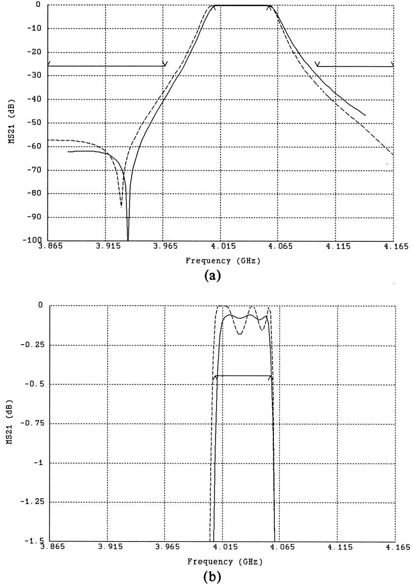
Fig. 13. Modeling of the notch in the |S_{21}| response of the HTS parallel coupled-line filter. In order to model the notch we introduced an additional inductor between the input and output of the filter. The analytical/empirical model response is shown as a dashed line. The EM simulated response is shown as a solid line. (a) Response of the overall band. (b) Passband details of the response.
