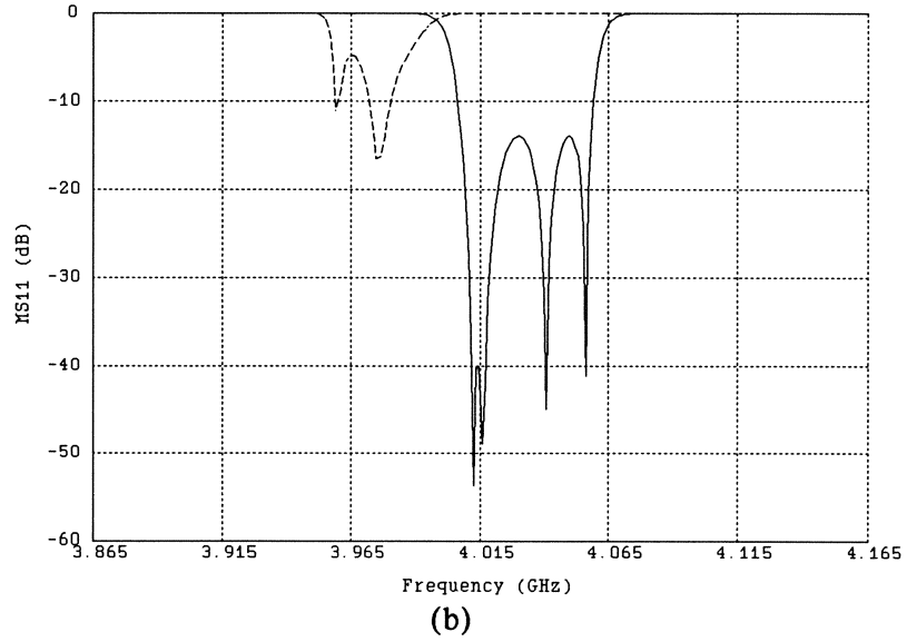
Fig. 2. The optimal solutions (solid lines) of (a) |S_{21}| and (b) |S_{11}| obtained using OSA90/hope. The corresponding em simulation results are shown as dashed lines. V indicate upper and \Lambda indicate lower specifications.
