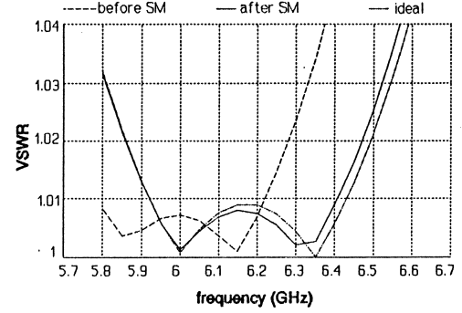
Fig. 7. VSWR response of a two-section waveguide transformer simulated by HFSS before and after 10 SM optimization iterations. Also shown is the optimal ideal response. The frequency is in GHz.
