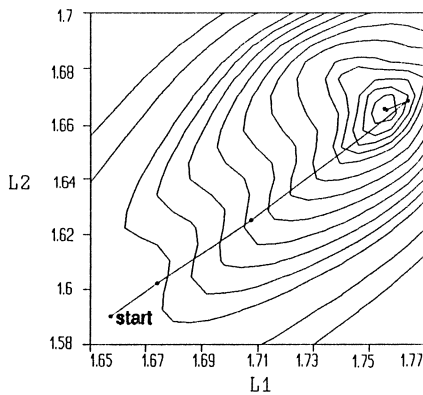
Fig. 10. The \ell_1 contours of multi-point parameter extraction of the two-section waveguide transformer. The parameter extraction has a unique solution.
