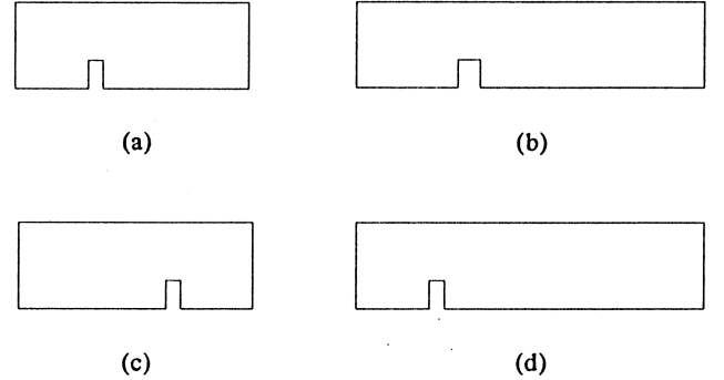
Fig. 2. Various evolutions of a microstrip line with a slit: (a) the initial geometry, (b) proportional expansion of the whole structure along the x axis, (c) only the location of the slit in the fixed line is allowed to change, and (d) only the segment to the right of the slit is allowed to expand.
