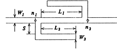
Fig. 6. Double folded stub filter.
