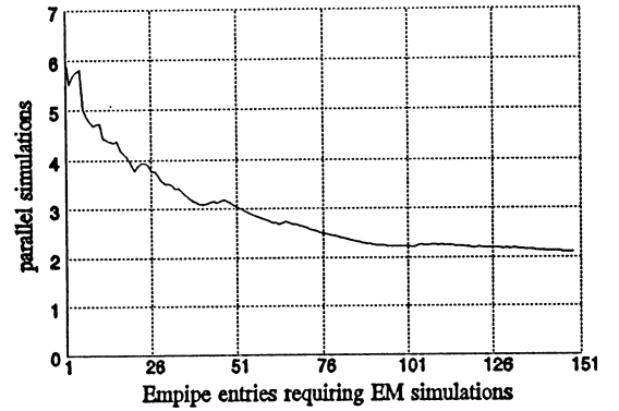
Fig. 4. The cumulative average number of EM analyses run in parallel.
