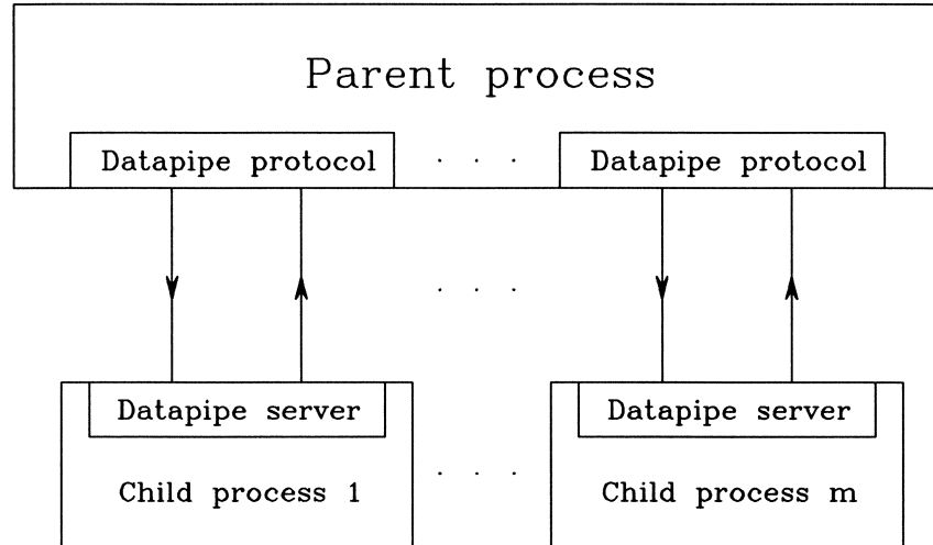
Fig. 1. Datapipe schematic.
