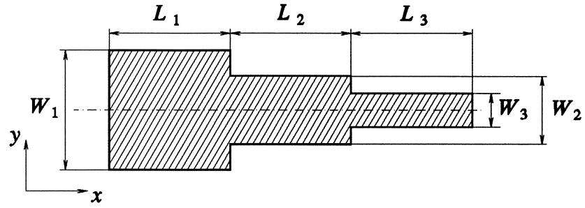
Fig. 3. 3-section microstrip impedance transformer. The widths of the sections W_1 , W_2 and W_3 are the designable parameters. The lengths L_1 , L_2 and L_3 are fixed.
