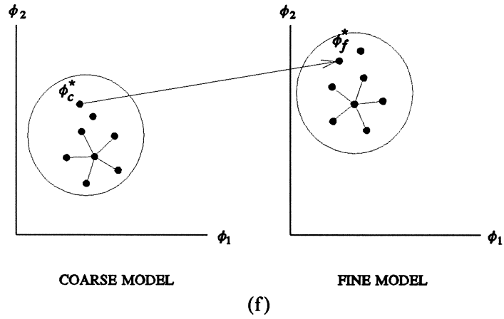
Fig. 2 (cont.) (d) Use inverse transformation to obtain the fine model point \phi_f^{m+1} = \phi_f^7 , which in this case did not satisfy (5). (e) Perform coarse model parameter extraction again to obtain \phi_c^7 . (f) Use the new projection model to obtain \phi_f^* = \phi_f^8 .
