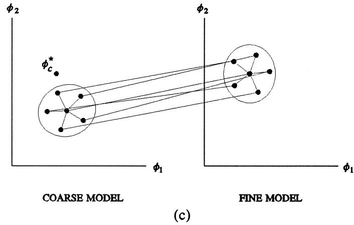
Fig. 2. Illustration of the SM process. (a) Coarse model optimization to obtain \phi_c^* . (b) Generation of five additional perturbations around \phi_f^1 = \phi_c^* . (c) Perform coarse model parameter extraction to match the fine model responses.
