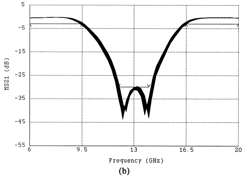
Fig. 14. The |S_{21}| Monte Carlo sweep obtained using the fine model after (a) coarse model yield optimization and (b) SM yield optimization. 250 outcomes are used for yield estimation and 200 outcomes are used in yield optimization.
