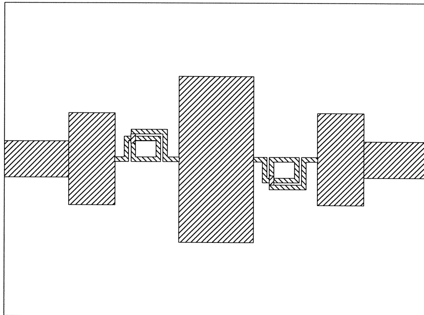
Fig. 4. Low-pass microstrip filter. The thickness and dielectric constant of the substrate are 25 mils and 9.8, respectively.
