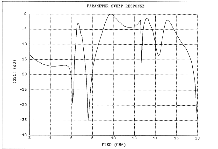
Fig. 3. |S_{21}| in dB vs. frequency for the rectangular structure.
