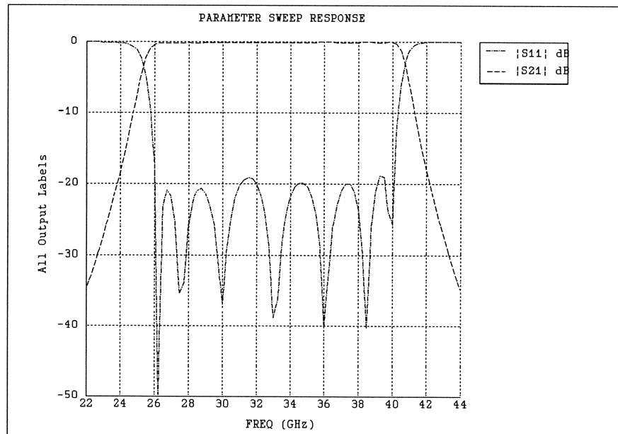
Fig. 10. 26–40 GHz interdigital capacitor filter simulation after optimization. All the optimization variables have been rounded to 0.1 mil resolution.
