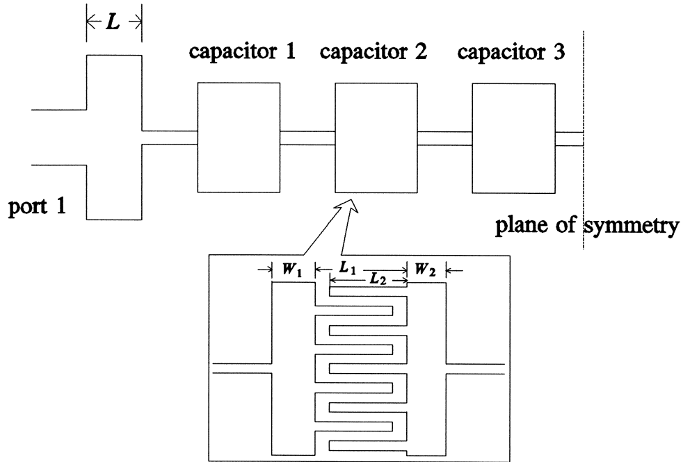
Fig. 9. The 26–40 GHz interdigital capacitor filter. The dielectric constant is 2.25. Substrate thickness and shielding height are 10 and 120 mils, respectively. The optimization variables include L , and L_1 , L_2 , W_1 , W_2 for each capacitor, totalling 13.
