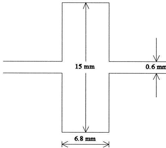
Fig. 2. A microstrip rectangular structure [9]. The thickness and dielectric constant of the substrate are 0.635 mm and 10.0, respectively.
