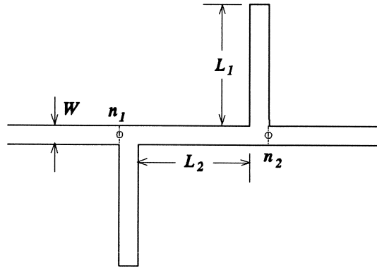
Fig. 6. Double folded stub microstrip structure for band-stop filter applications.
