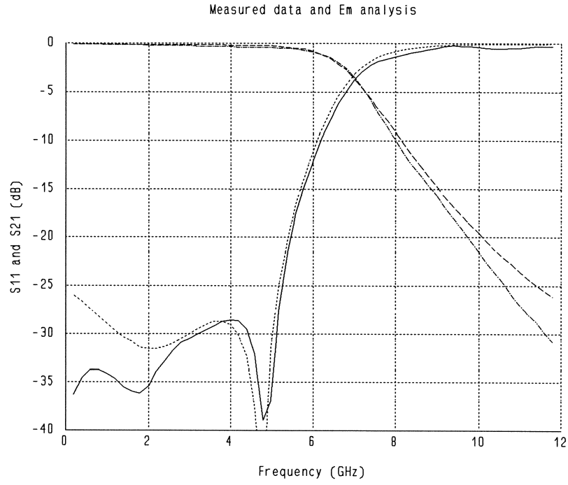
Fig. 5. EM simulation and measurements of the low-pass filter: (---) simulated |S_{11}| , (-.-.-) measured |S_{11}| , (.....) simulated |S_{21}| , and (—) measured |S_{21}| .
