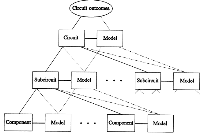
Fig. 1 Schematic diagram illustrating multilevel modeling for yield-driven optimization. Solid and dotted lines distinguish between exact and approximate responses.
