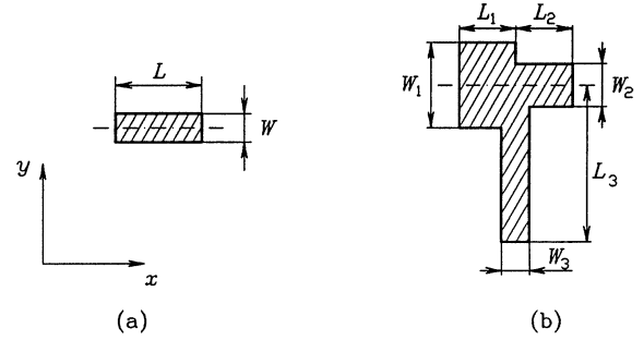
Fig. 4 Parameters of (a) the feedback microstrip line and (b) the microstrip T-junctions.
