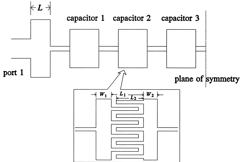
Fig. 5. 26-40 GHz interdigital capacitor filter. Dielectric constant is 2.25. Substrate thickness and shielding height are 10 and 120 mils, respectively. The optimization variables include L , and L_1 , L_2 , W_1 , W_2 for each capacitor, totalling 13.
