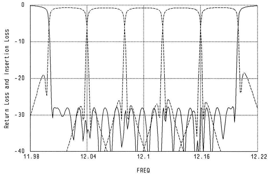
Fig. 8 Multiplexer responses after minimax optimization with the full set of 75 variables.
