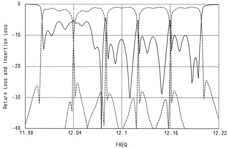
Fig. 6 Multiplexer responses after minimax optimization with 10 variables: spacings and channel input transformer ratios. This result hardly improved upon the starting point shown in Fig. 5.
