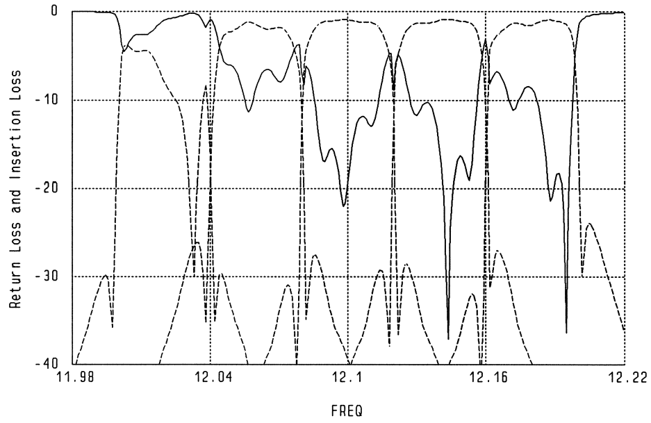
Fig. 5 Multiplexer responses at the starting point.
