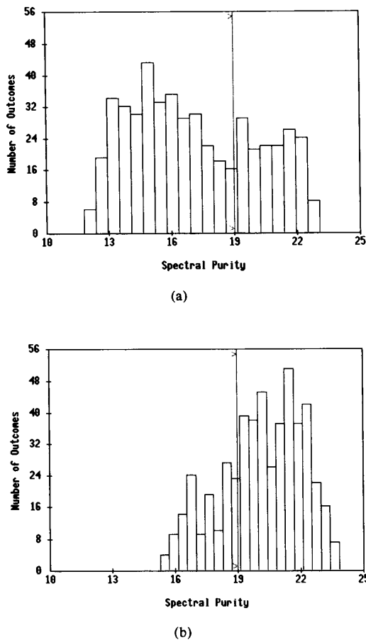
Fig. 3. Histogram of spectral purity of the frequency doubler based on 500 outcomes (a) before yield optimization and (b) after yield optimization. The specification is shown by a vertical line.
