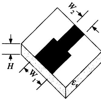
Fig. 5. Microstrip step junction.
