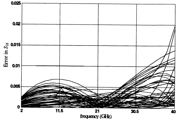
Fig. 6. Modulus of the complex S_{21} error for the MSM-FSMSM microstrip step junction.
