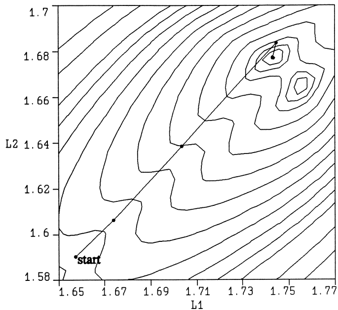
Fig. 8. The l_1 contours of the parameter extraction problem for the two-section waveguide transformer. The symmetry between the variables L_1 and L_2 produces two local minima. Consequently the result of parameter extraction is not unique.
