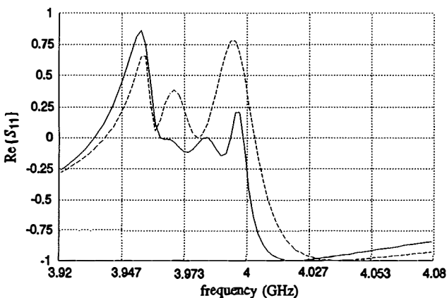
Fig. 8. \text{Re}(S_{11}) simulated using the empirical model (—) and em (---) at the starting point after applying the FSM algorithm. This starting point is now ready for regular parameter extraction.
