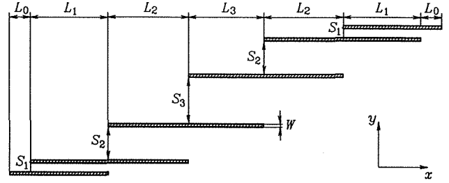
Fig. 2. The structure of the HTS filter.
