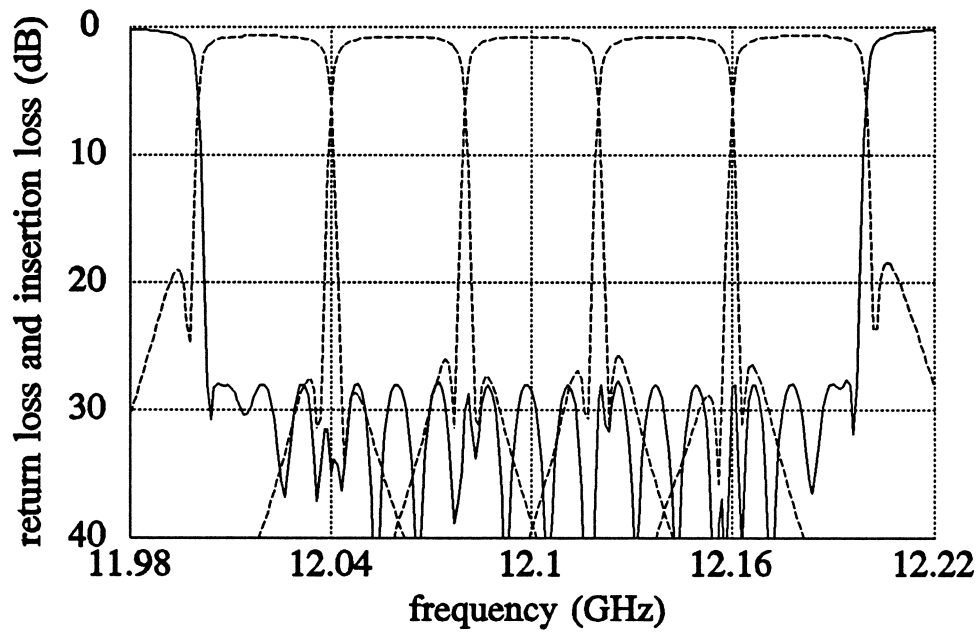
Fig. 6.7 Multiplexer responses after the minimax optimization with the full set of 75 variables, showing the common port return loss (—) and the individual channel insertion losses (-----).
