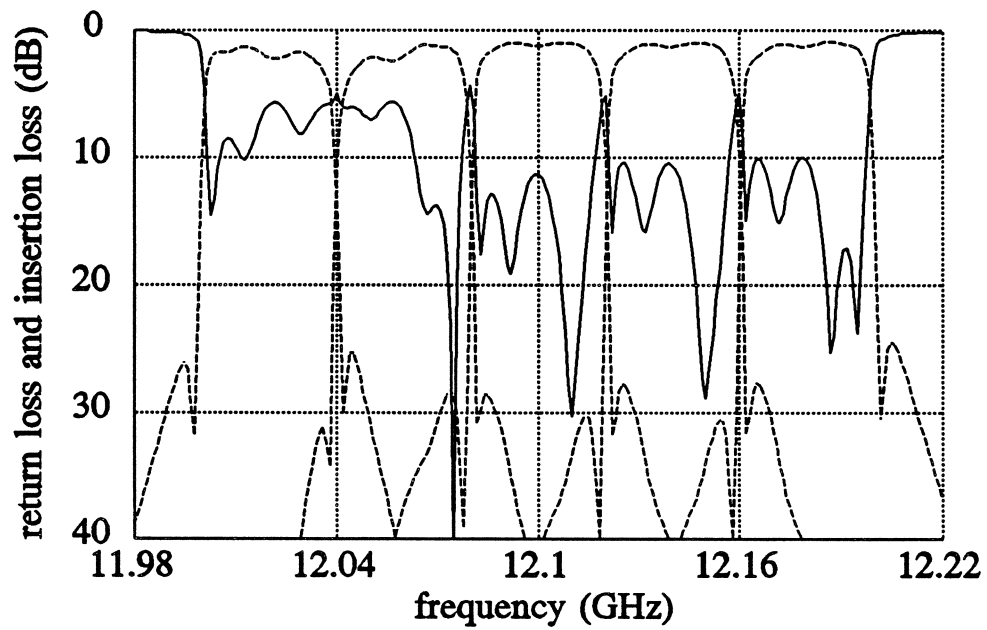
Fig. 6.4 Multiplexer responses after the minimax optimization with 10 variables: spacings and channel input transformer ratios; the common port return loss (—) and the individual channel insertion losses (-----). This result hardly improved upon the starting point shown in Fig. 6.3.
