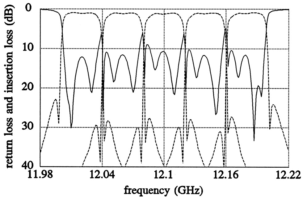
Fig. 6.5 Multiplexer responses after the one-sided Huber optimization with 10 variables: spacings and channel input transformer ratios; the common port return loss (—) and the individual channel insertion losses (-----). This result is significantly better than the minimax solution shown in Fig. 6.4.
