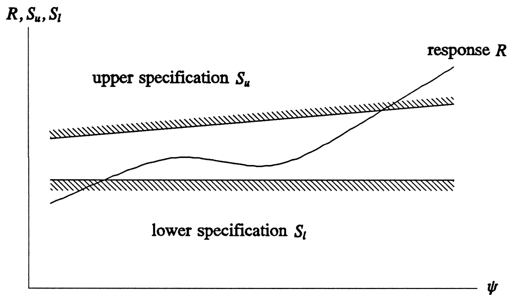
Fig. 2.1(a) Circuit response with upper and lower specifications.
