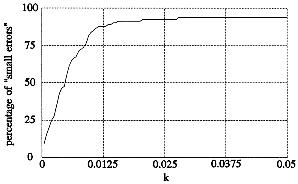
Fig. 4.4. Percentage of "small errors" for the FET gate lead inductance L_G versus the threshold k .
