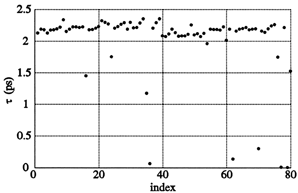
Fig. 4.2 Run chart of the extracted FET time-delay \tau [13].
