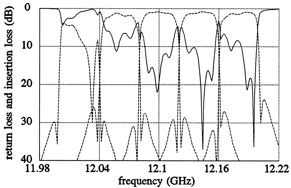
Fig. 6.3 Multiplexer responses at the starting point, showing the common port return loss (—) and the individual channel insertion losses (-----).
