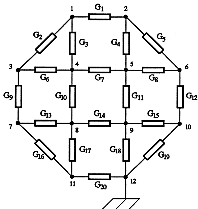
Fig. 5.1 The resistive mesh circuit [11,13,57].
