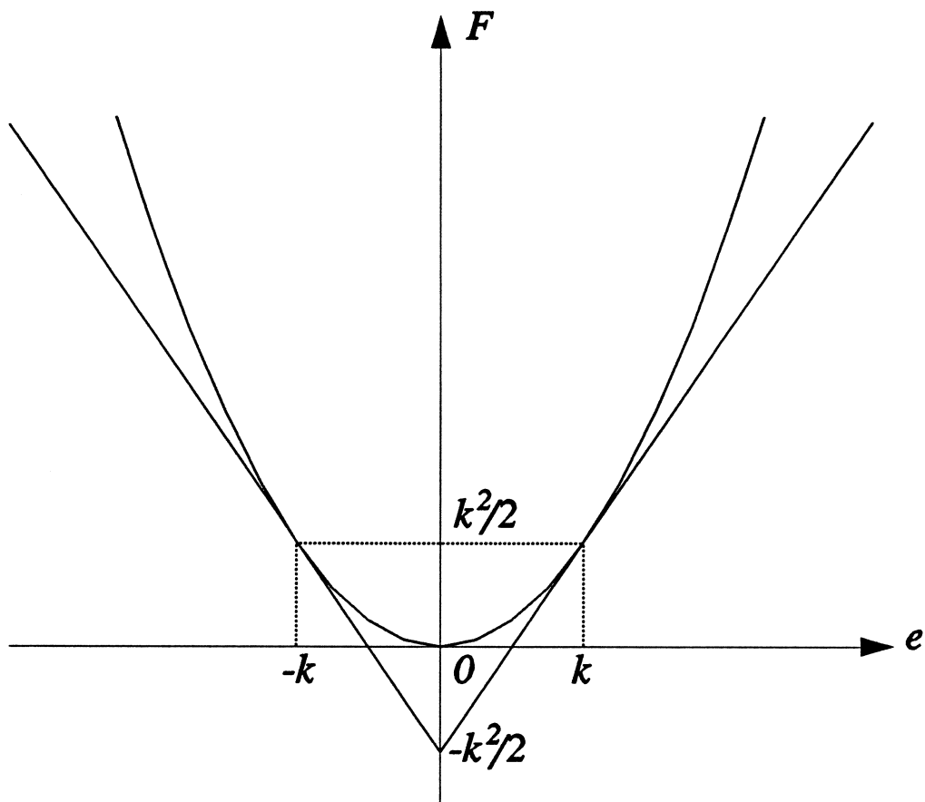
Fig. 2.5(a). The \ell_1 and \ell_2 functions. The \ell_1 function is rescaled and shifted in accordance with the corresponding part in the Huber function. It has the form F = k|e| - k^2/2 . The \ell_2 function has the form F = e^2/2 .
