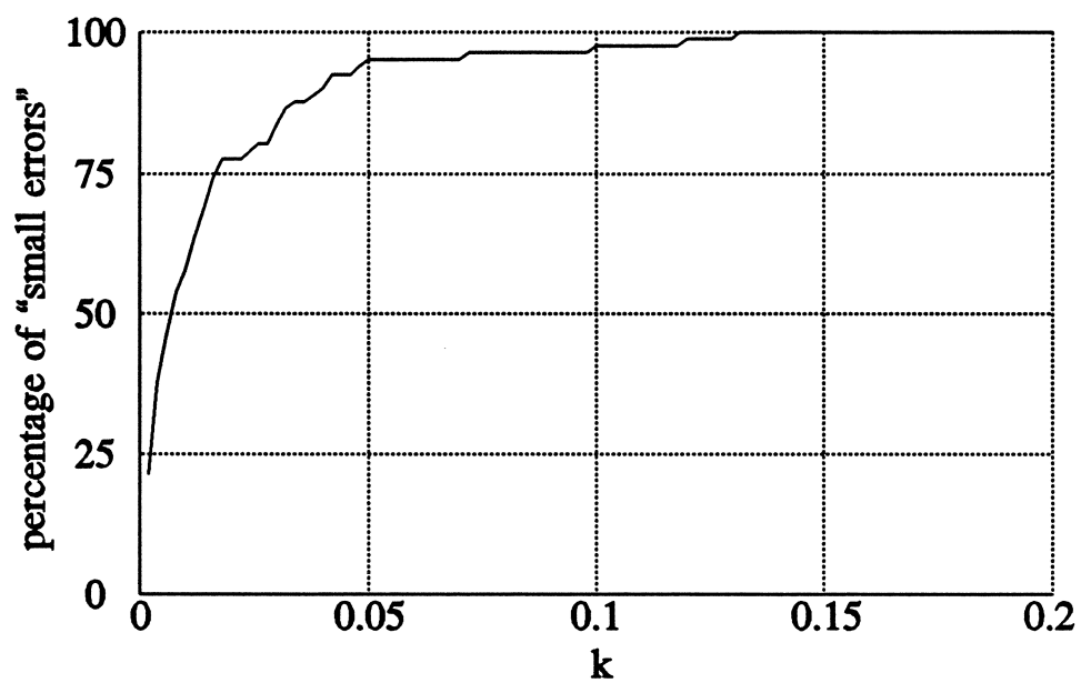
Fig. 4.5. Percentage of "small errors" for the FET model parameter C_{10} versus the threshold k .
