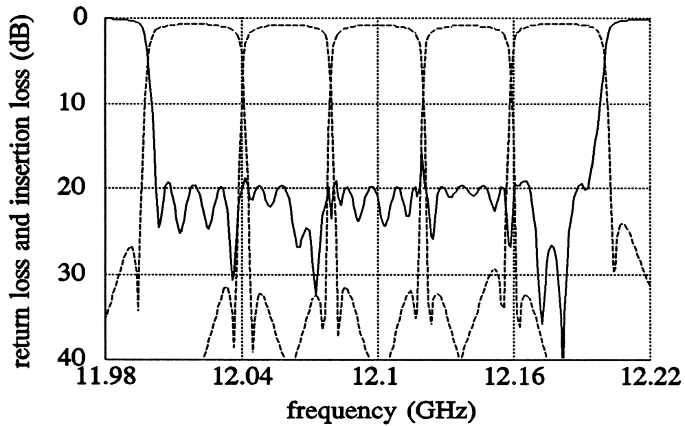
Fig. 6.6 Multiplexer responses after the one-sided Huber optimization with 45 variables, showing the common port return loss (—) and the individual channel insertion losses (-----).
