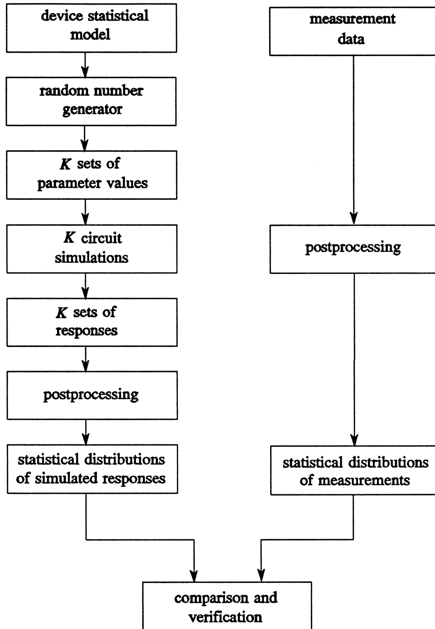
Fig. 4.1 Statistical model verification using Monte Carlo simulation [34].
