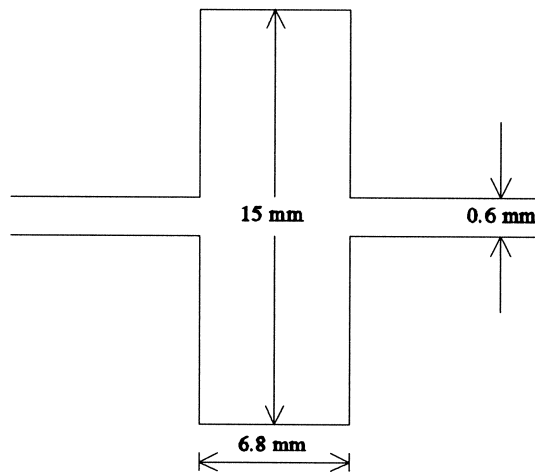
Fig. 2. A microstrip rectangular structure [9]. The thickness and dielectric constant of the substrate are 0.635 mm and 10.0, respectively.
