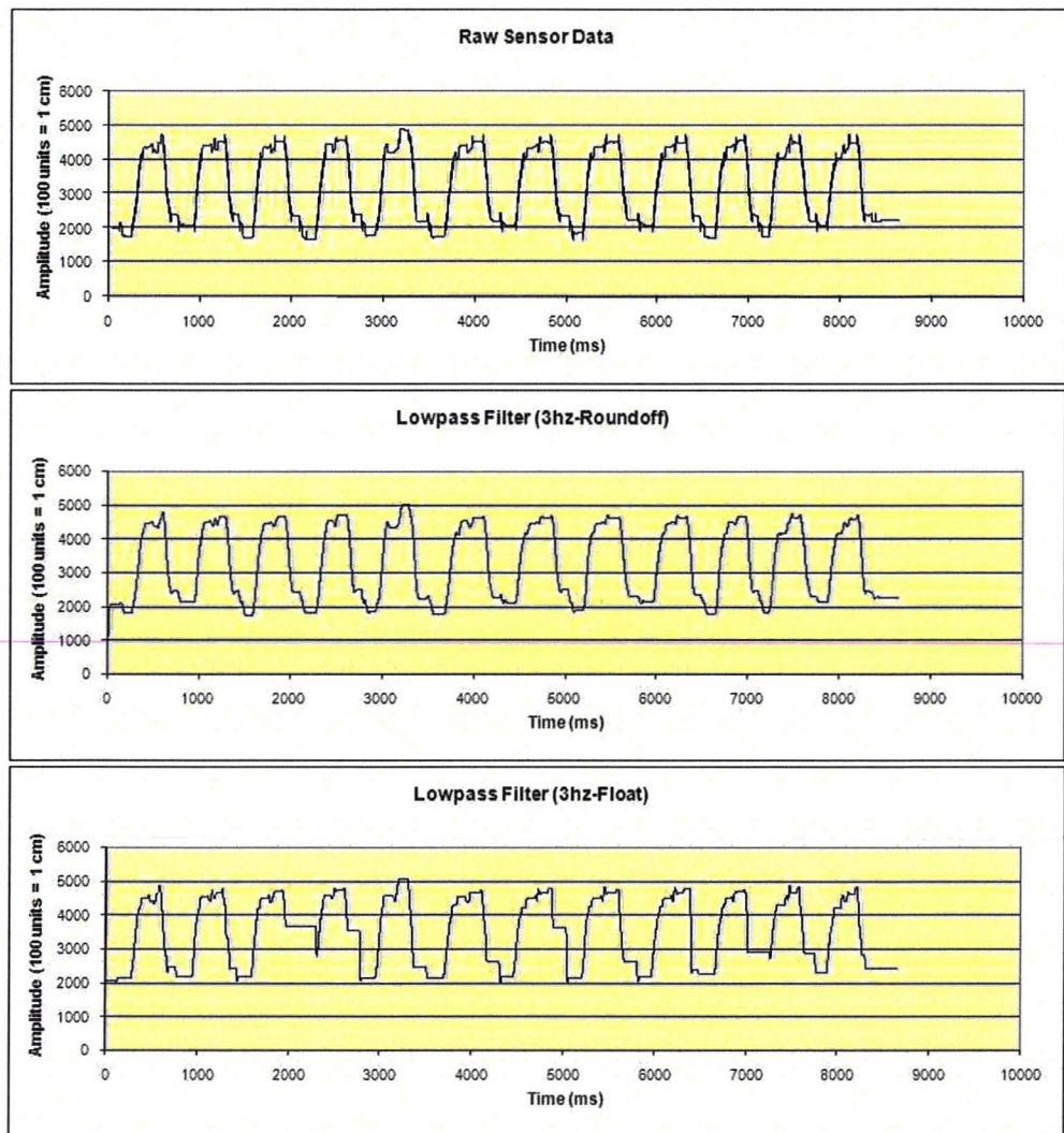
Figure 4.8: The effects of rounding on filtered data.
