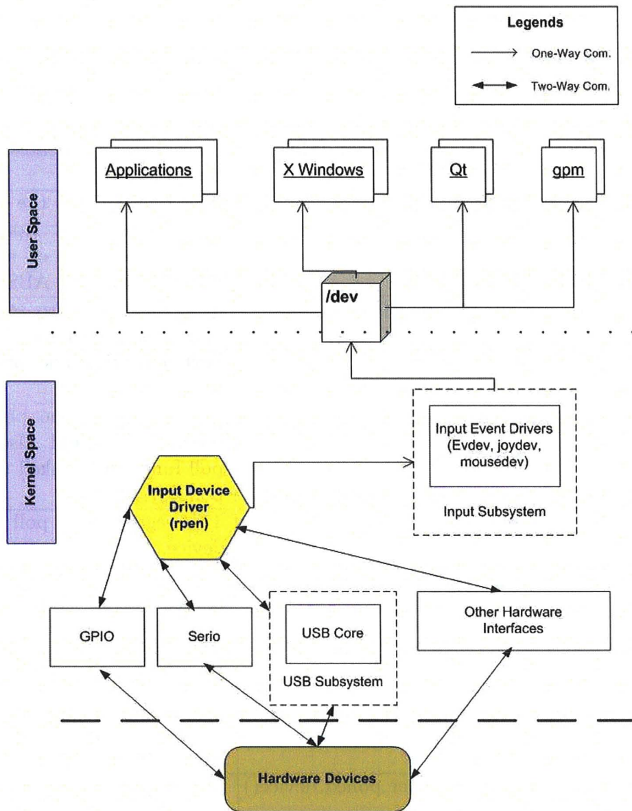
Figure 3.5: Linux input subsystem; adapted from [Ven08].
