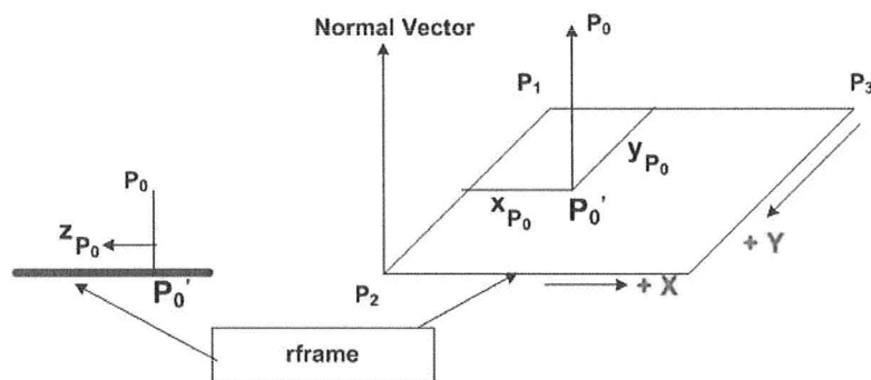
Figure 3.13: Calculating a point on the generic rframe.
