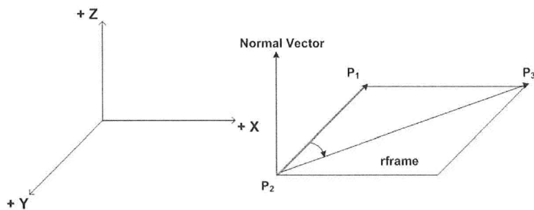
Figure 3.12: An example of a generic rframe, showing the normal vector.
