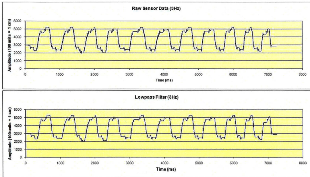
Figure 4.4: Raw sensor data and effect of 3Hz lowpass filter on the data.
