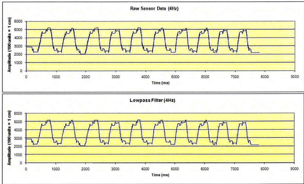
Figure 4.5: Raw sensor data and effect of 4Hz lowpass filter on the data.
