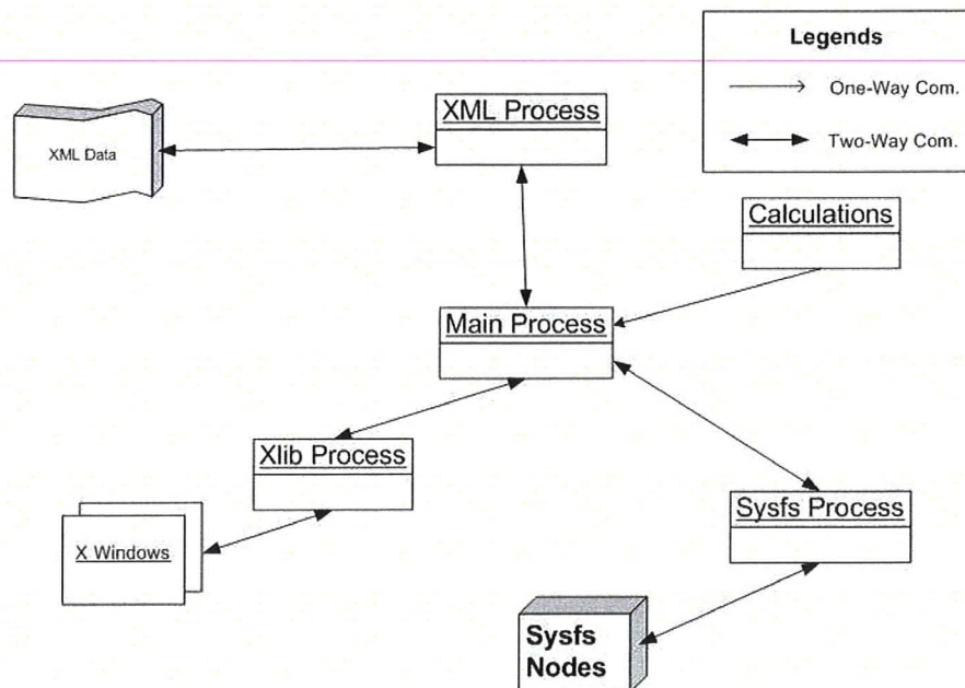
Figure 3.25: Feedback daemon structure.
