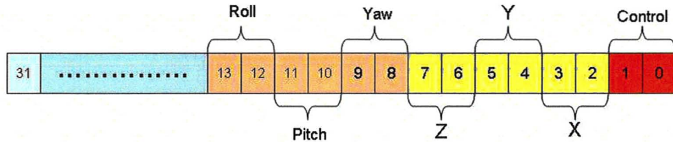
Figure 3.8: Format of Wintracker data sent to host system.
