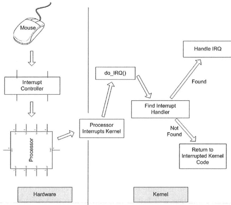
Figure 3.2: Interrupt handling process [Lov05].
