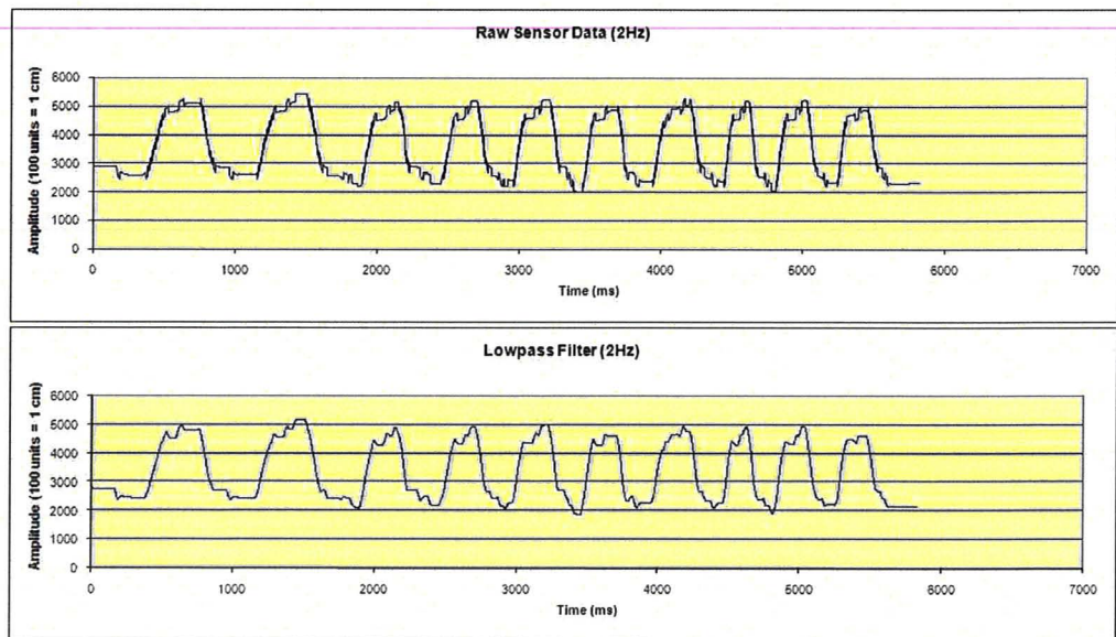
Figure 4.3: Raw sensor data and effect of 2Hz lowpass filter on the data.
