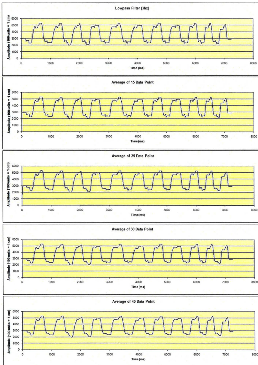
Figure 4.6: The effects of averaging of 15, 25, 30, and 40, 3Hz lowpass filter data points.
