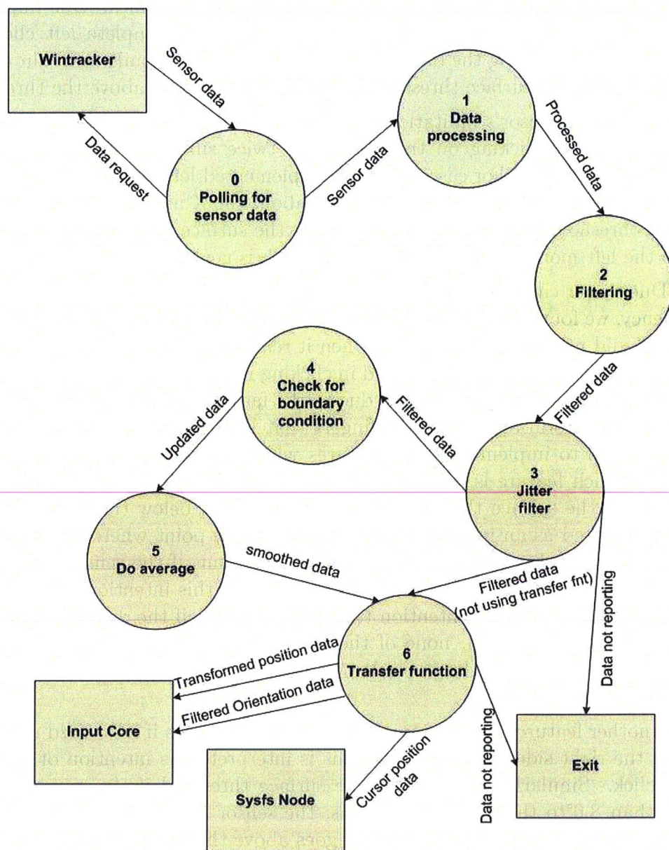
Figure 3.16: Dataflow diagram of the rpen device driver, showing dataflow on each sensor data read.
