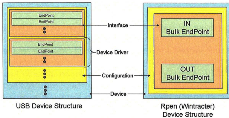
Figure 3.4: Structure of a generic USB device along with the structure of Wintracker, that is used for rpen.
