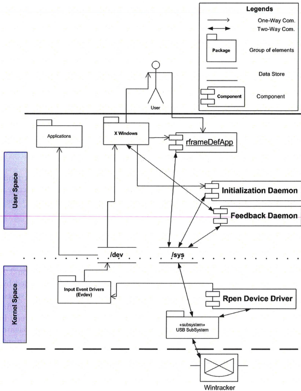
Figure 3.10: High level rpen design.
