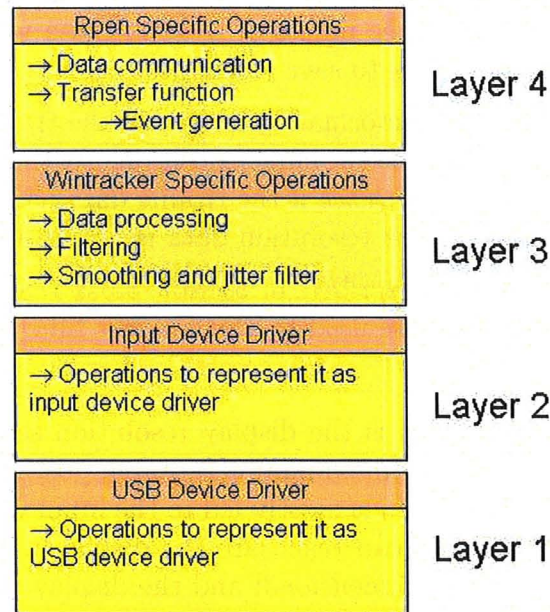
Figure 3.14: Rpen device driver structure.
