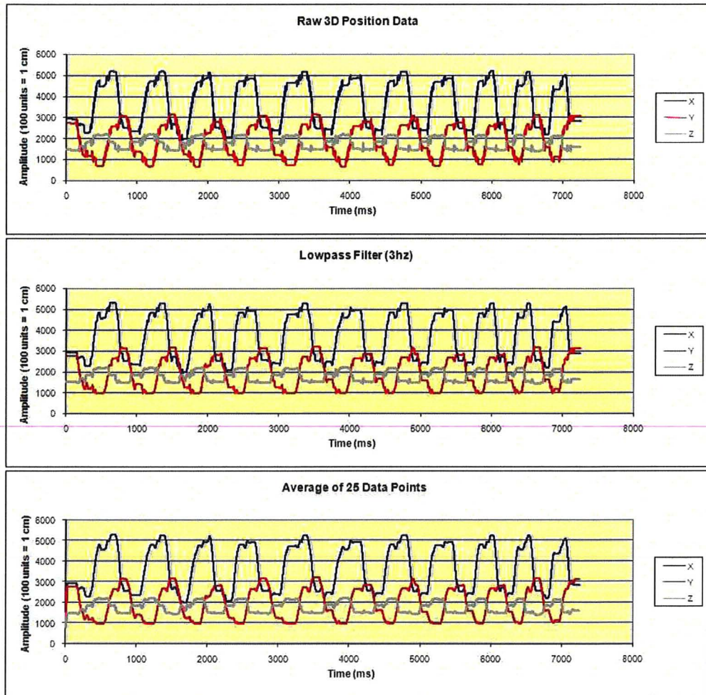
Figure 4.7: The effects of the lowpass filter, jitter filter and averaging on raw sensor data. Rpen implements this scheme to filter out noise and smooth filtered data.
