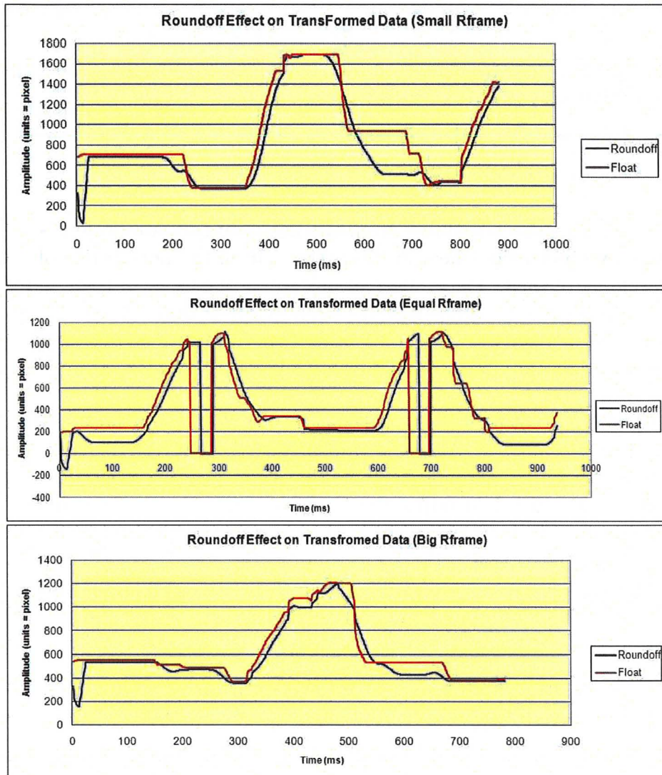
Figure 4.9: Graphs showing roundoff effect on final 3D cursor position data. Also showing roundoff effect depending on rframe resolution. The first one uses a smaller rframe in relative to display resolution. In the second one, a equal sized rframe is used. In the third scenario, a bigger rframe is utilized.
