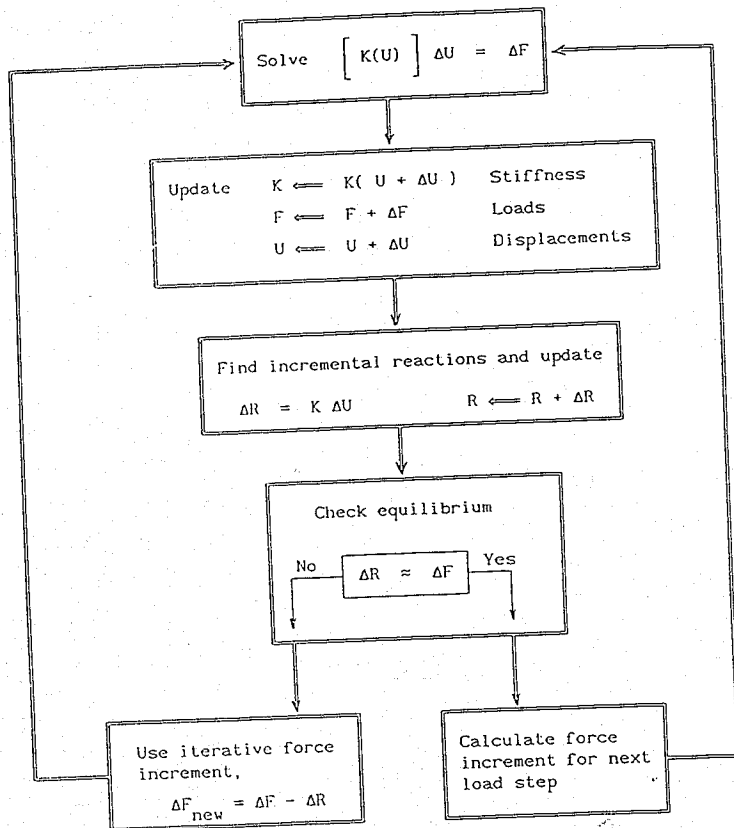
Figure 4.1 Typical incremental nonlinear algorithm
