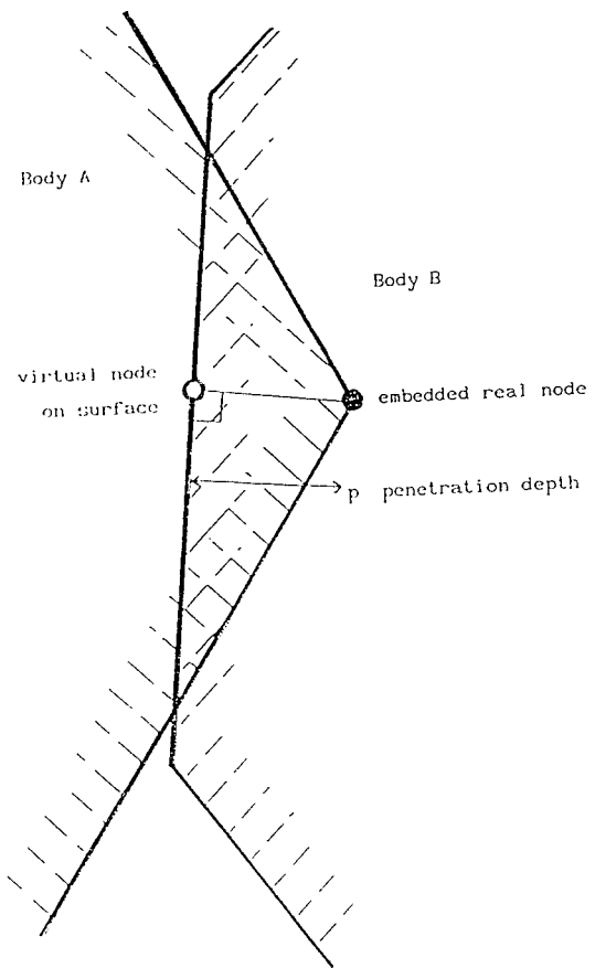
Figure 4.4 Determination of penetration depth
