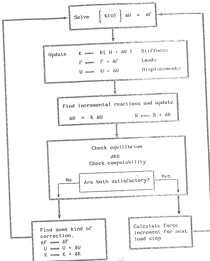
Figure 4.2 Typical incremental contact algorithm
