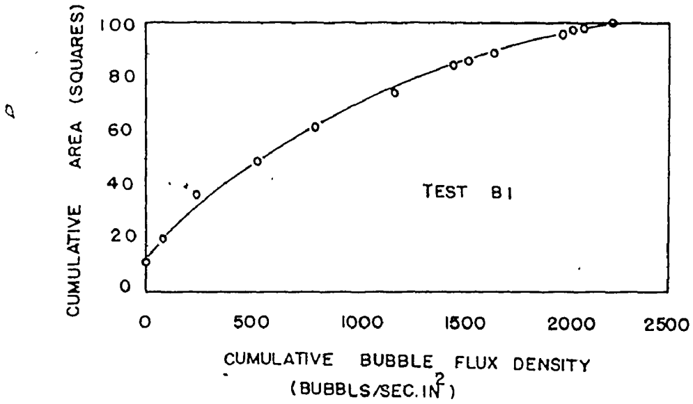
Figure (53) Cumulative Bubble Flux Density Versus Cumulative Area
