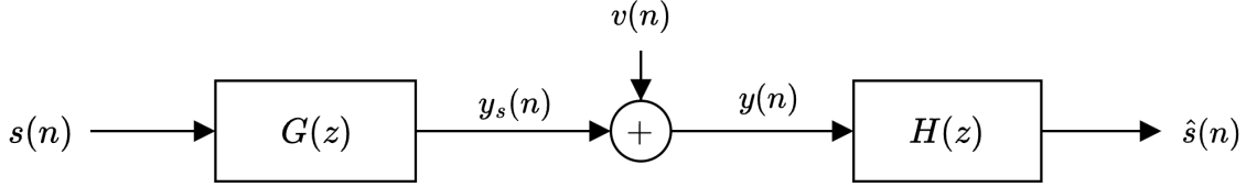
Figure 2.4: Block diagram for blind deconvolution, which attempts to produce reproduce the unknown input, s(n) , to an unknown system G(z) , from the measured system output, y(n) , including additive noise v(n) , using a filter, H(z)
