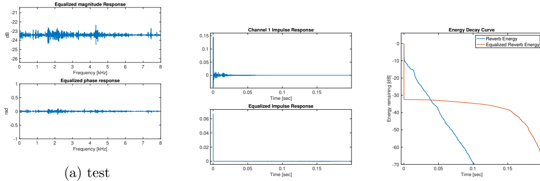
Figure A.1: Delay-and-Predict dereverberation performance with multichannel linear prediction order p2 = L/(M - 1) , where L is the FIR RIR length and M is the number of channels. Figure 3.2 shows the common source whitening filter used.
