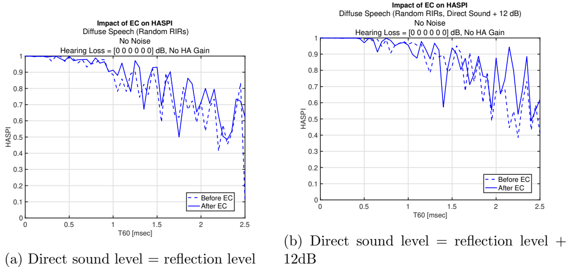
Figure A.11: Impact of EC algorithm on speech intelligibility (using HASPI) as a function of varying amounts of synthetic reverb, noise-free.
