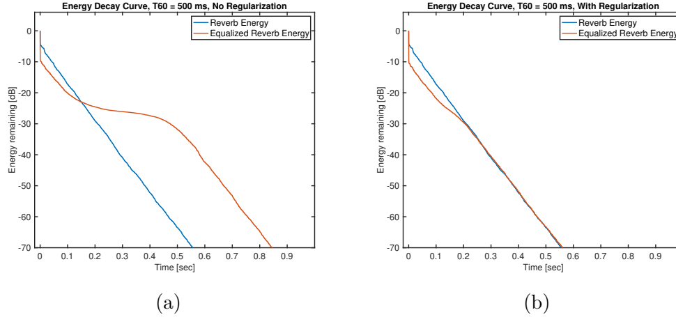
Figure 4.20: Impact of autocorrelation matrix regularization on dereverberation performance. Prediction orders were p_2 = 2667 and p_1 = 10000 (i.e., according to T60_{\max} = 500 m sec for M = 4 and f_s = 16 kHz).
