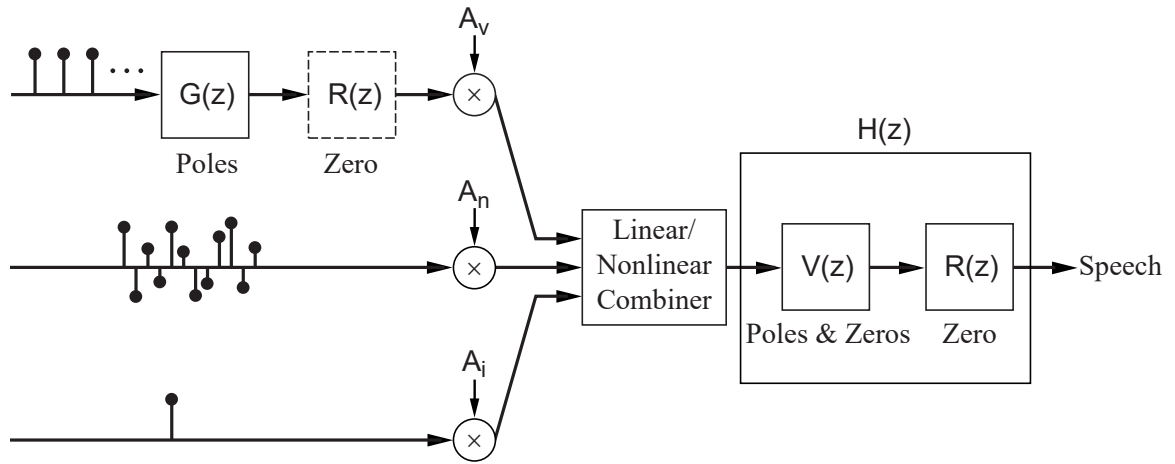
Figure 1.6: Discrete-time speech production model. Used with permission of Pearson, Figure 4.20 from Quatieri (2002) ©2002.
