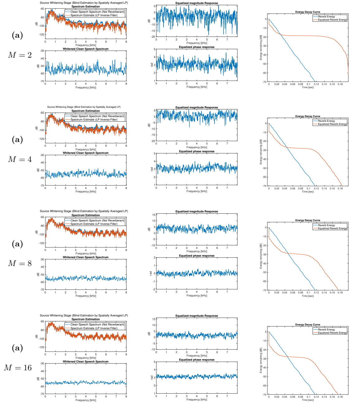
Figure 3.8: Impact of number of microphones M on DAP dereverberation performance. Source whitening prediction order was p_1 = 1.25 \cdot p_2 \cdot (M - 1) and MC-LP order was p_2 = N60/(M - 1) . Source Whitening stage was performed on reverberant speech (i.e., blind estimation). RIRs were synthetically generated exponentially decaying Gaussians.
