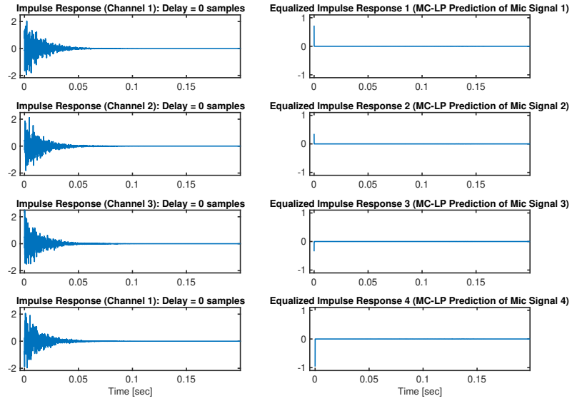
Figure 3.12: Vector-valued EIR performance prior to linear combiner with no time delay between channels (i.e., time aligned).
