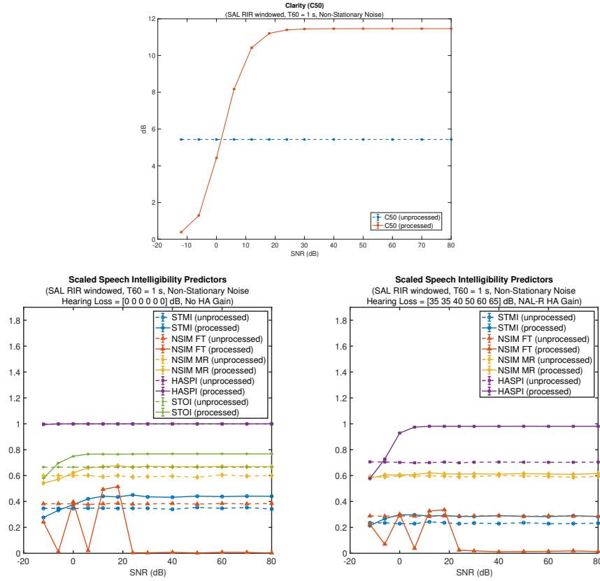
Figure 4.25: Evaluation of delay-and-predict dereverberation performance with autocorrelation regularization in the presence of noise as a function of SNR. RIRs were generated by applying a variable decay-rate exponential window to a measured RIR (The SAL room from the MYRiAD database, T_{60} = 2.2 s) to set T_{60} = 1 s. Noise was a multichannel recording of non-stationary noise (Cafeteria babble noise from the HRIR database).
