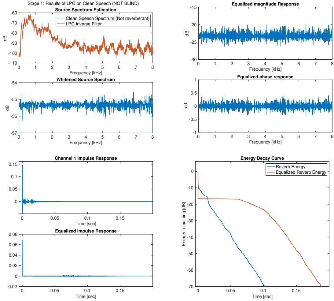
Figure A.6: Delay-and-Predict dereverberation performance with source whitening prediction order p_1 = 1000 and multichannel linear prediction order p_2 = N60/(M - 1) .
