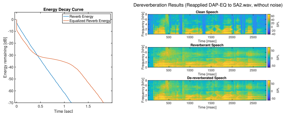
Figure 3.7: DAP Equalizer performance (EDC and Spectrogram) with the source-whitening filter computed using reverberant speech (i.e., blind)
