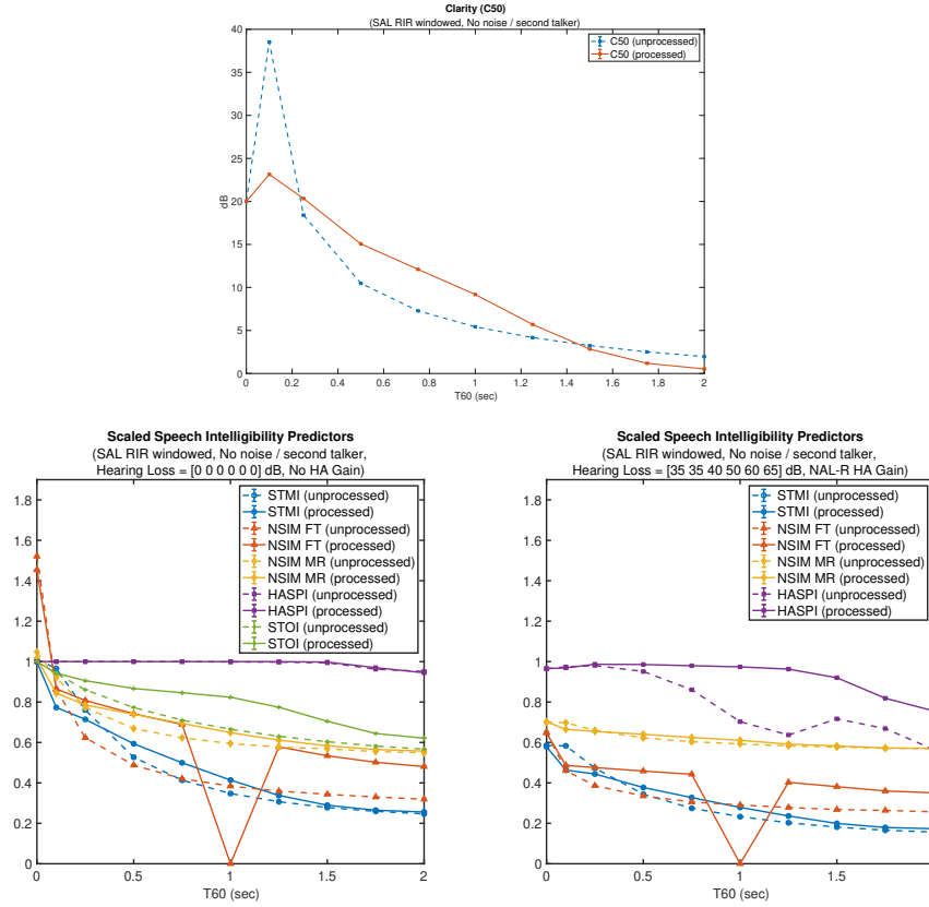
Figure 4.19: Evaluation of delay-and-predict dereverberation performance as a function of T60. Prediction orders were p_2 = 2667 and p_1 = 10000 (i.e., set according to T60_{\max} = 500 msec for M = 4 and f_s = 16 kHz). RIRs were generated by applying a variable decay-rate exponential window to a measured RIR (The SAL room from the MYRiAD database, T60 = 2.2 s) to control T60. No Noise or Interfering talker were included.
