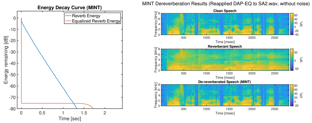
Figure 3.5: MINT Equalizer performance (EDC and Spectrogram)
