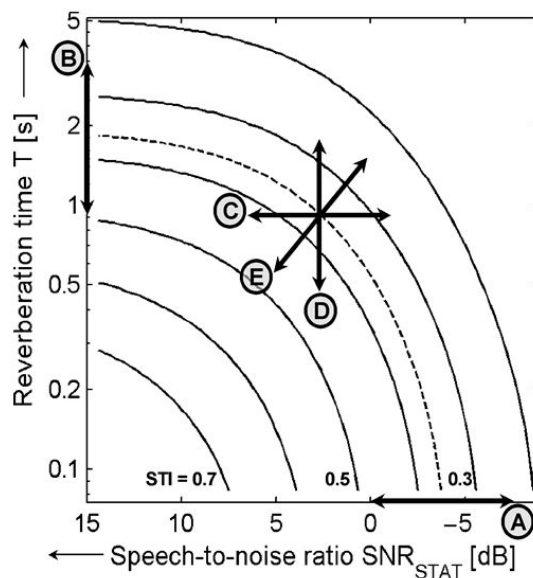
Figure 1.7: Mapping of SNR and reverberation time (synthetically generated exponentially decaying Gaussian RIRs) to STI. The dotted contour denotes the speech recognition threshold (SRT). Used with permission of American Speech-Language-Hearing Association, Figure 1 from George et al. (2010) ©2010; permission conveyed through Copyright Clearance Center, Inc.
