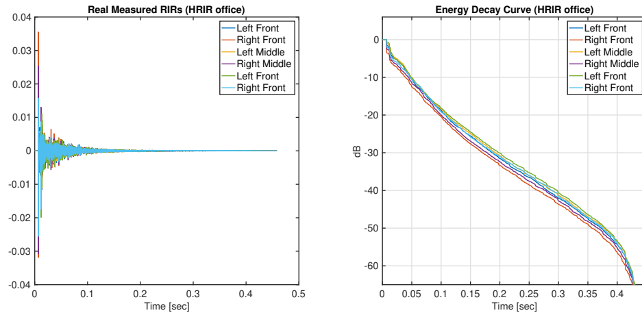
Figure 4.1: EIR and EDC of the HRIR database office II room
