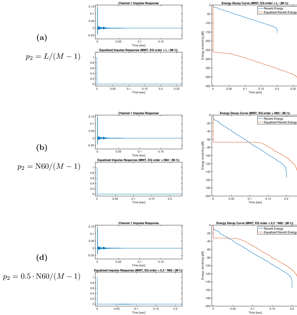
Figure 3.1: MINT equalizer performance for various equalizer orders. Equalizer orders ( p_2 ) are quantified relative to the actual length of the FIR channel ( L ) and the number of samples corresponding to the T60 of the channel ( N60 = T60 \cdot \text{sample rate} )
