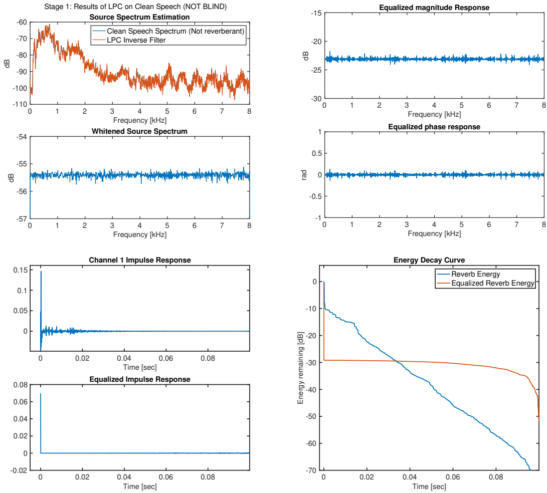
Figure A.7: Delay-and-Predict dereverberation performance with source whitening prediction order p_1 = p_2 \cdot (M - 1) and multichannel linear prediction order p_2 = N_{60}/(M - 1) . I.e., The source whitening filter order is the same as the effective MINT filter order.
