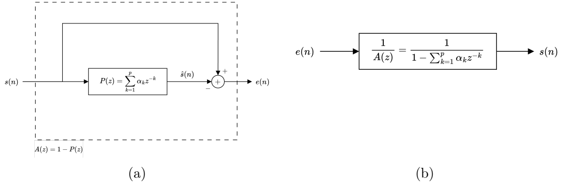
Figure 1.10: Block diagram for LP prediction-error filter, A(z) (a), and LP inverse filter, \frac{1}{A(z)} (b)
