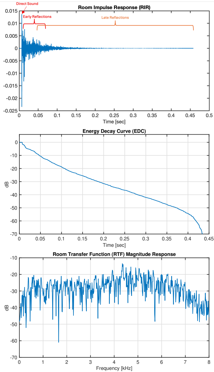
Figure 1.1: Example of a room impulse response (RIR), energy decay curve (EDC, defined in Equation 1.4) and room transfer function (RTF) magnitude response. RIR is the “office II” room from the HRIR database (Kayser et al. , 2009).
