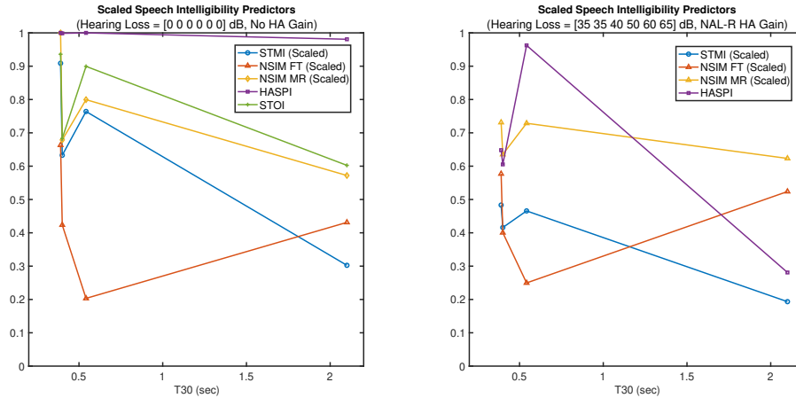
Figure 4.9: Impact of practical reverberation (several real measured RIRs) on SI predictors with and without hearing loss. NAL-R linear hearing aid amplification included in hearing loss case for metrics that including modeling of hearing loss. Scaling applied to NSIM and STMI values to better view all metrics on the same plot.
