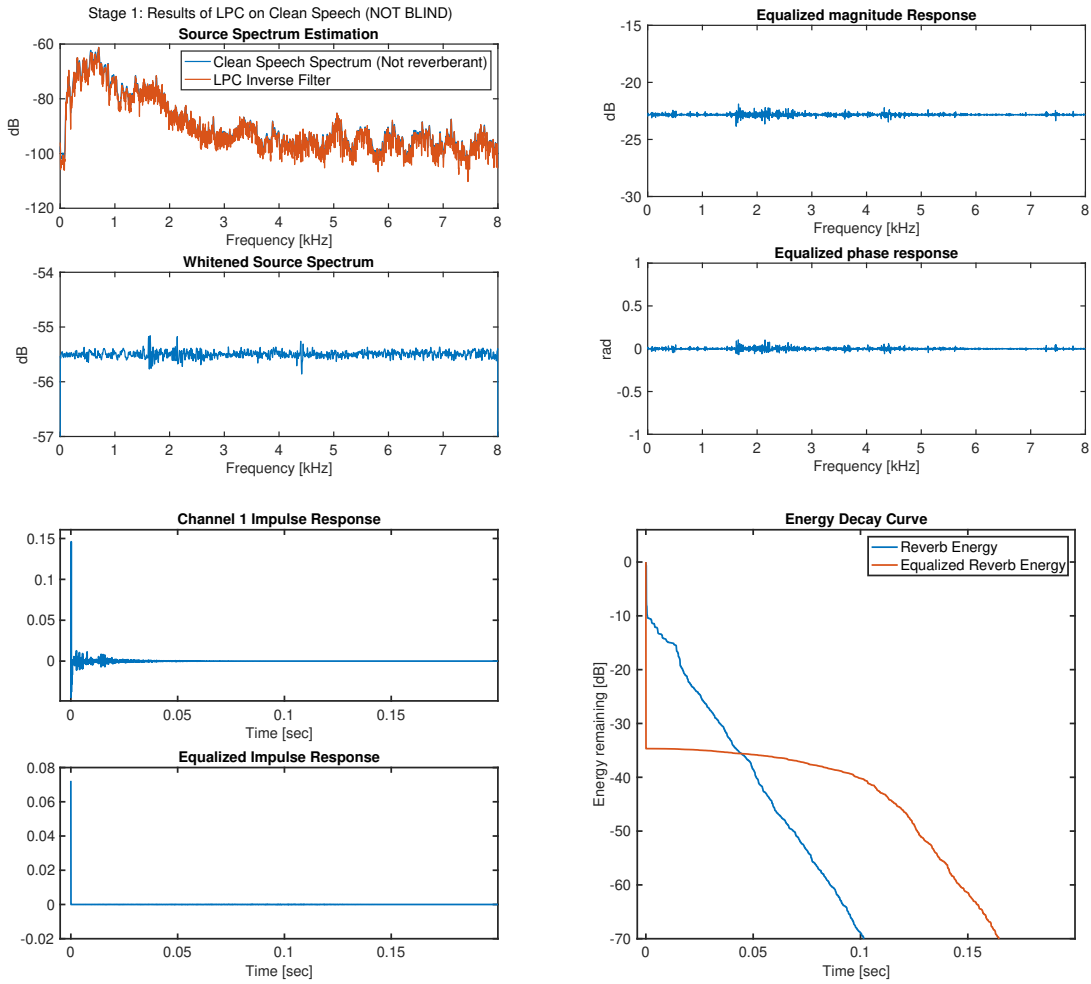
Figure A.8: Delay-and-Predict dereverberation performance with source whitening prediction order p_1 = 2 \cdot p_2 \cdot (M - 1) and multichannel linear prediction order p_2 = N_{60}/(M - 1) . I.e., The source whitening filter order is twice the effective MINT filter order.
