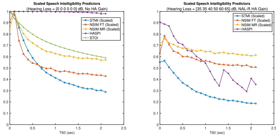
Figure 4.12: Impact of practical reverberation (SAL room from MYRiAD database exponentially truncated to control T60) on SI predictors with and without hearing loss. NAL-R linear hearing aid amplification included in hearing loss case for metrics that including modeling of hearing loss. Scaling applied to NSIM and STMI values to better view all metrics on the same plot.
