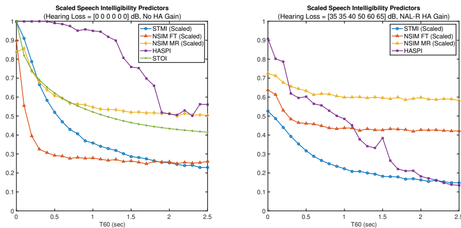
Figure 4.8: Impact of synthetic reverberation (exponentially decaying gaussian RIRs) on SI predictors with and without hearing loss. NAL-R linear hearing aid amplification included in hearing loss case for metrics that including modeling of hearing loss. Scaling applied to NSIM and STMI values to better view all metrics on the same plot.
