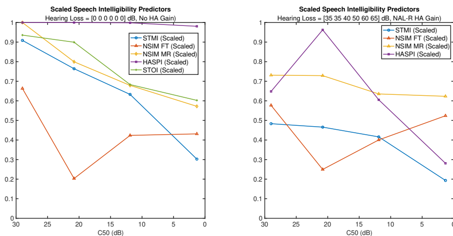
Figure 4.10: Relationship between SI predictors and C50 (Figure 4.9 replotted against C50)
