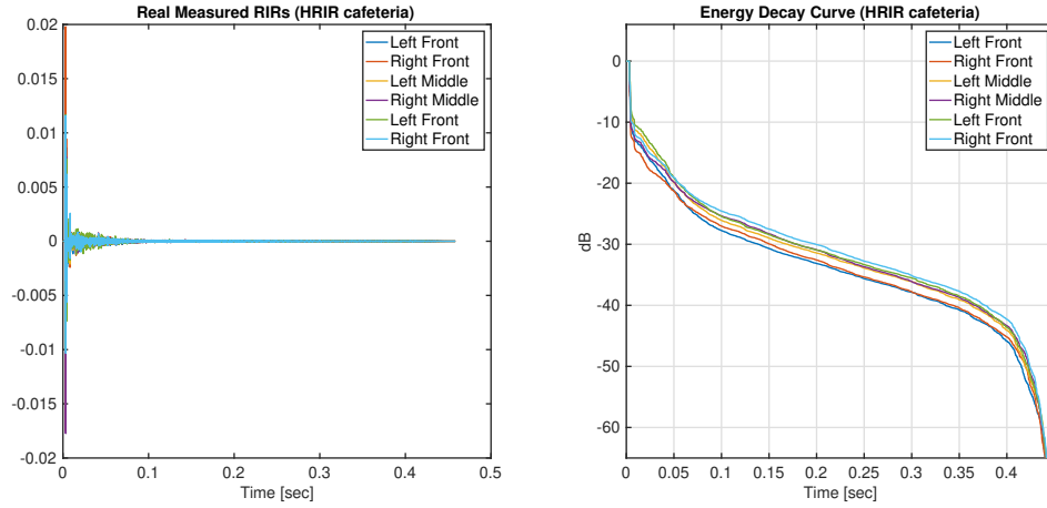
Figure 4.3: EIR and EDC of the HRIR database cafeteria room
