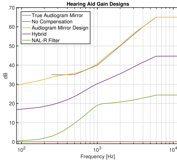
Figure 4.5: Hearing aid gains used in evaluation. The audiogram corresponds to IEC 60118-15 Moderate HL Moderately Sloping Group (Bisgaard et al. , 2010), and NAL-R refers to the gain proposed by Byrne and Dillon (1986).
