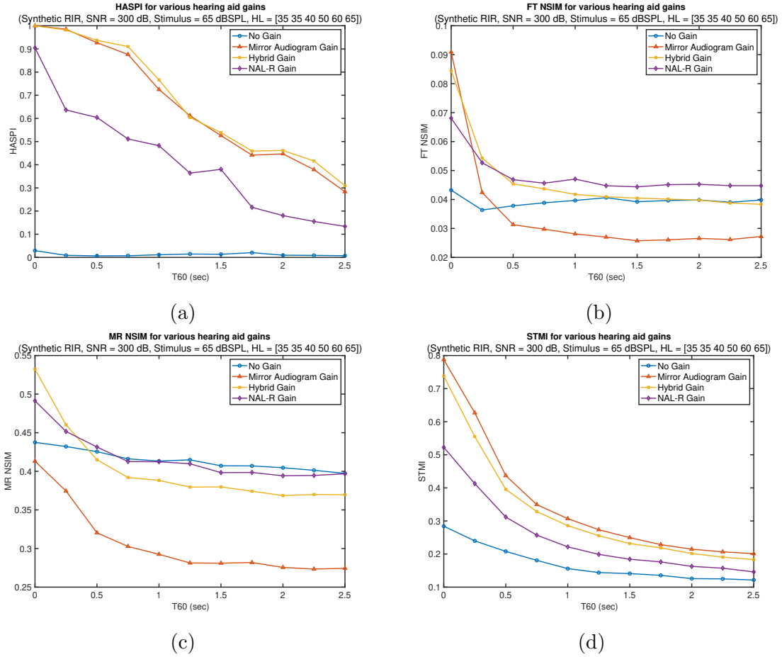
Figure 4.6: Comparison of perceptual benefit of four different linear hearing aid gains in the presence of reverberation. Moderate high frequency hearing loss used in the perceptual models (IEC 60118-15 Moderate HL, Moderately Sloping Group), and RIRs were generated synthetically.
