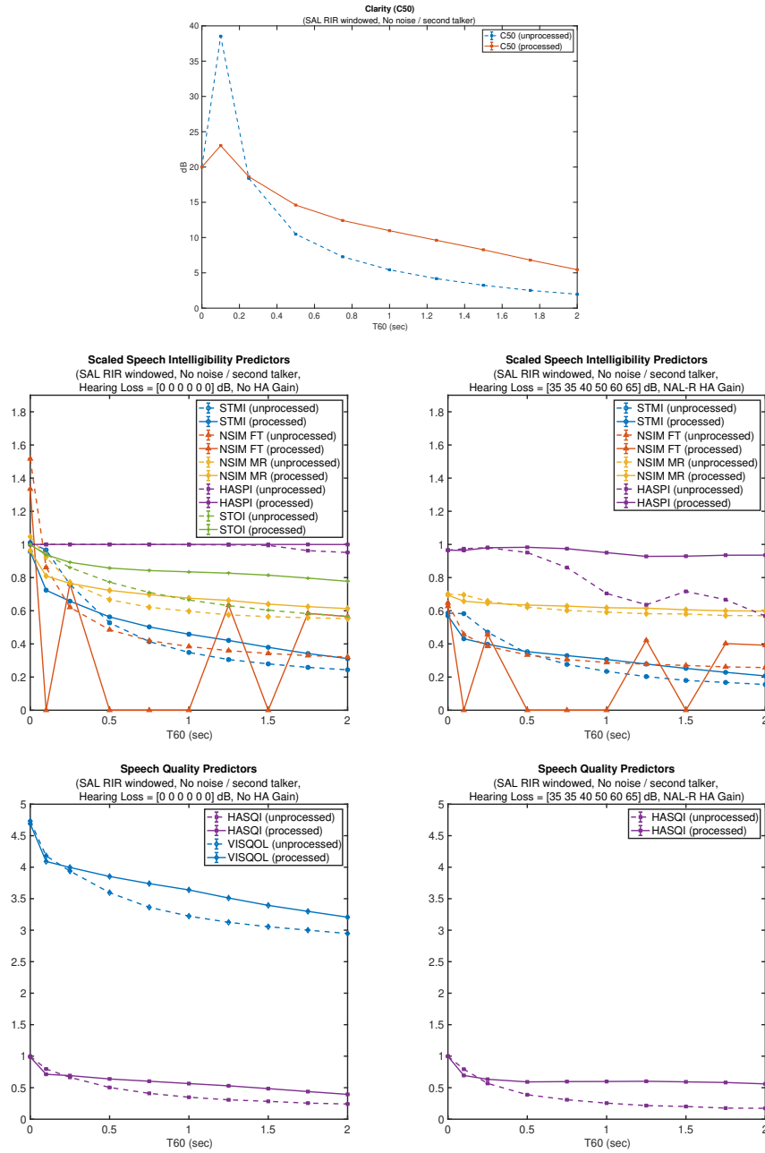
Figure 4.17: Evaluation of delay-and-predict dereverberation performance as a function of T60. Prediction orders were p_2 = 5333 and p_1 = 20000 (i.e., set according to T60_{\max} = 1 sec for M = 4 and f_s = 16 kHz). RIRs were generated by applying a variable decay-rate exponential window to a measured RIR (The SAL room from the MYRiAD database, T60 = 2.2 s) to control T60. No Noise or Interfering talker were included.
