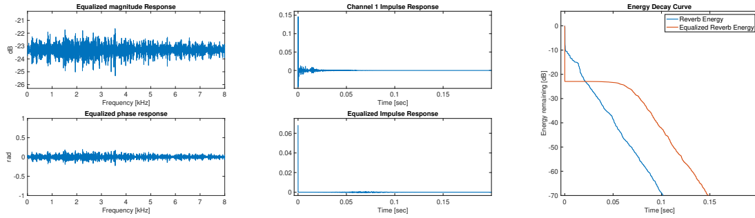
Figure A.4: Delay-and-Predict dereverberation performance with multichannel linear prediction order p_2 = 0.5 \cdot N_{60}/(M - 1) , where N_{60} is the number of samples corresponding to the T60 and M is the number of channels (i.e., More suboptimal with respect to the MINT condition based on T60 rather than the FIR RIR length). Figure 3.2 shows the common source whitening filter used.
