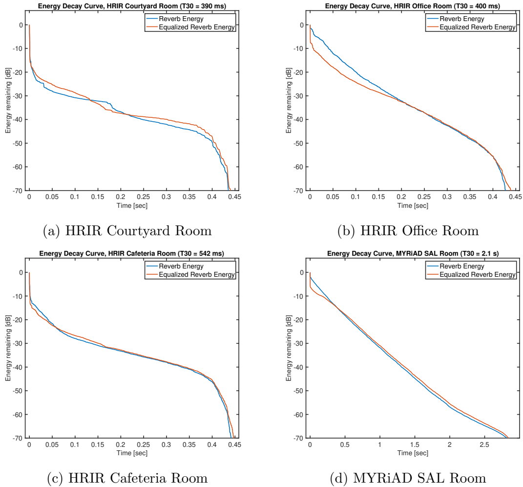
Figure 4.23: EDC performance results corresponding to a single iteration of the test results shown in Figure 4.22.
