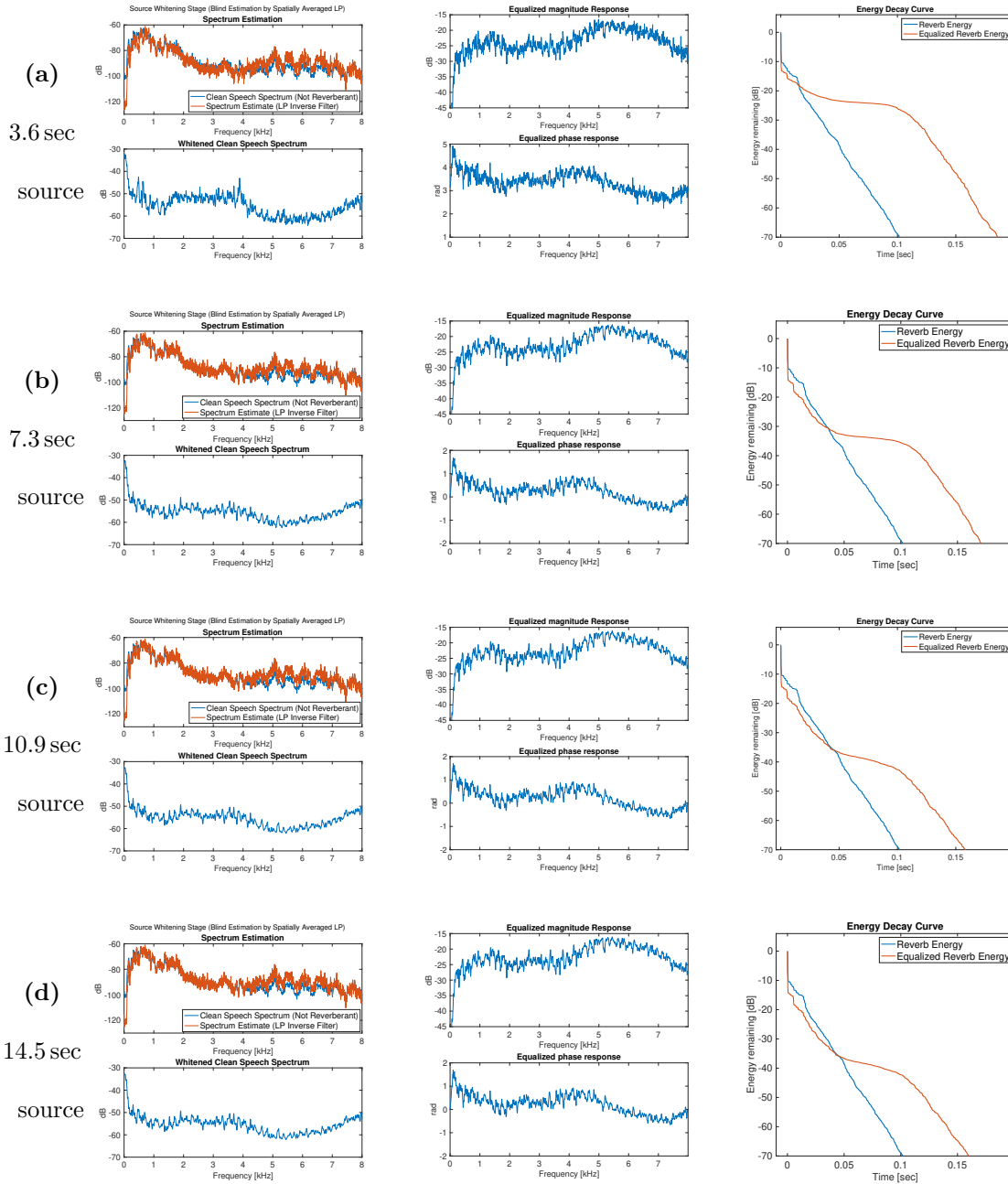
Figure 3.9: Impact of source data length on DAP dereverberation performance. In each case, the same 3.6 sec speech sample (58 ksamples at f_s = 16 kHz) was looped to a different data length to preserve the same spectrum. Source whitening prediction order was p_1 = 2 \cdot p_2 \cdot (M - 1) and MC-LP order was p_2 = N_{60}/(M - 1) . Source Whitening stage was performed on reverberant speech (i.e., blind estimation).
