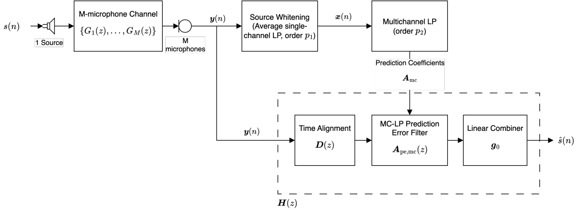
Figure 2.7: Block diagram for delay-and-predict dereverberation
