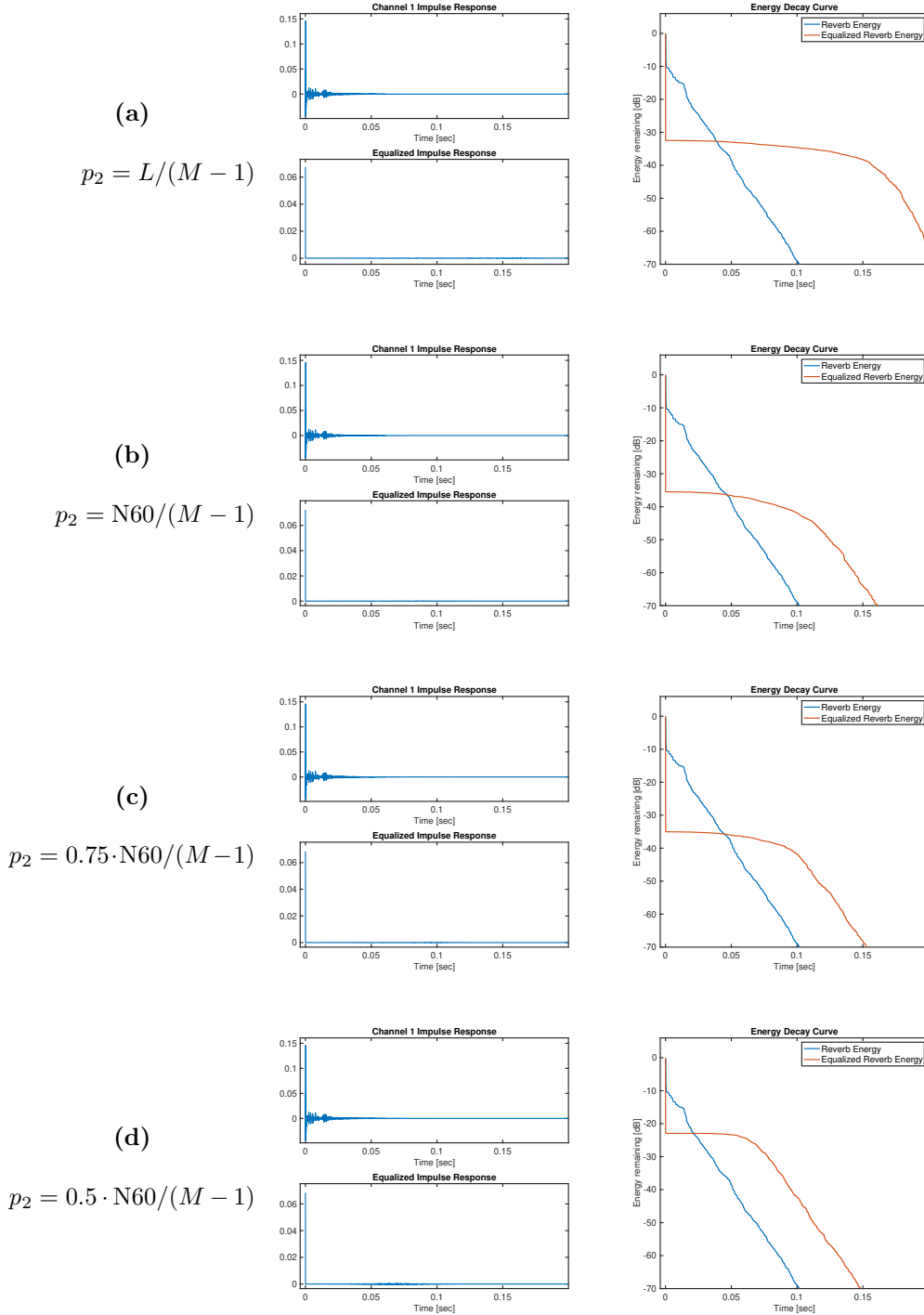
Figure 3.3: Impact of MC-LP order ( p_2 ) on DAP dereverberation performance. Prediction orders are quantified relative to the actual length of the FIR channel ( L ) and the number of samples corresponding to the T60 of the channel ( N60 ). Figure 3.2 shows the common source whitening filter used.
