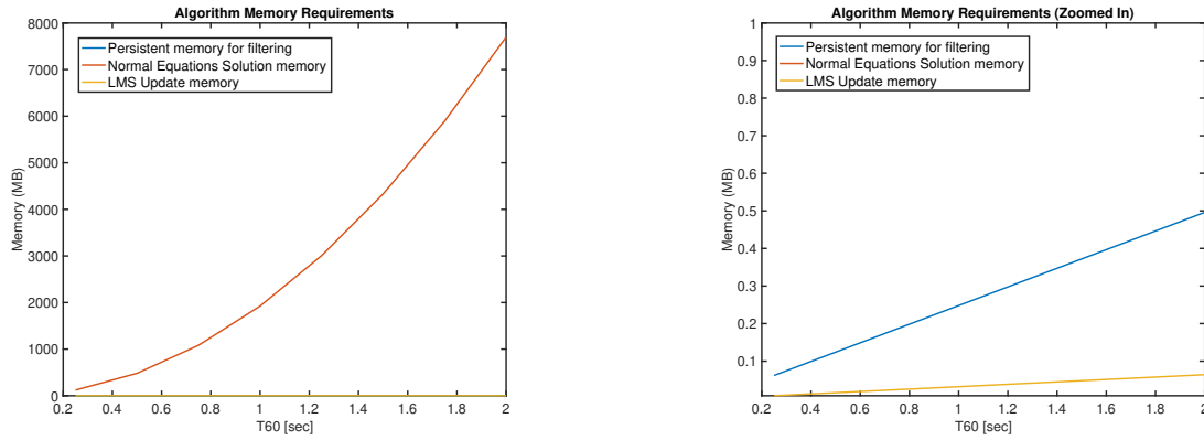
Figure 3.17: Analysis of the algorithmic memory requirements of Least Squares solution (could be temporary memory) and Inverse filter implementations (persistent memory) as a function of T60, For M=4 microphones, p_2 = 0.75 \cdot N_{60}/(M - 1) and p_1 = 1.25 \cdot p_2 \cdot (M - 1) . Memory requirements of LMS Solution also shown for comparison.
