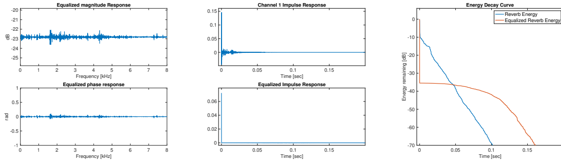
Figure A.2: Delay-and-Predict dereverberation performance with multichannel linear prediction order p_2 = N_{60}/(M - 1) , where N_{60} is the number of samples corresponding to the T60 and M is the number of channels (i.e., the MINT condition based on T60 rather than the FIR RIR length). Figure 3.2 shows the common source whitening filter used.
