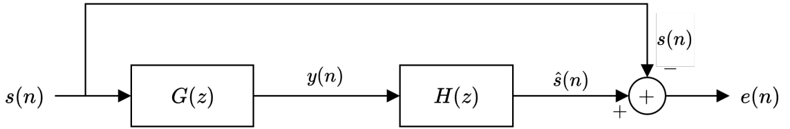
Figure 2.3: Block diagram for supervised inverse filtering / equalization, which attempts to reproduce the known input, s(n) , to an unknown system G(z) , from the measured system output, y(n) , using a filter, H(z)
