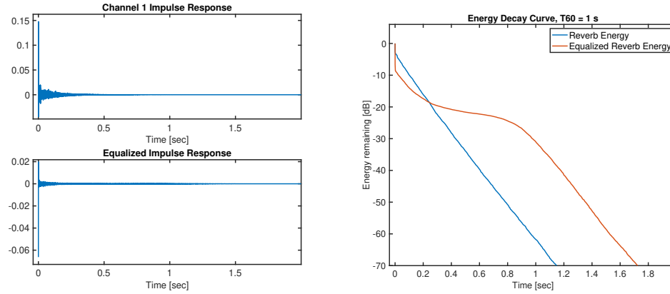
Figure 4.18: EDC and EIR performance from a single iteration of the results shown in Figure 4.17 for a T60 of 1 sec
