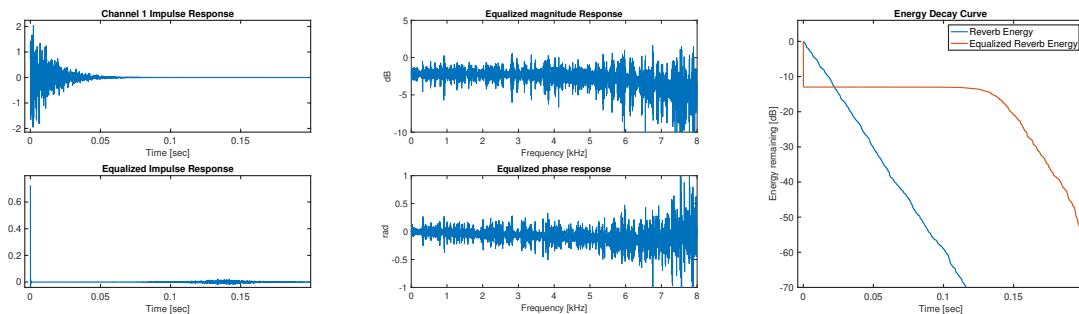
Figure 3.15: DAP dereverberation performance (after linear combiner) with an incremental 2-sample delay added to each channel (i.e., not time aligned).
