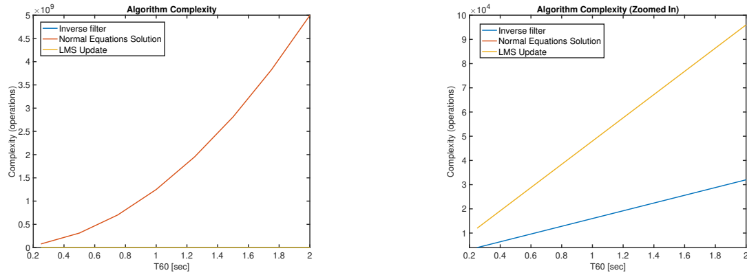
Figure 3.16: Analysis of the computational complexities of Least Squares solution and Inverse filter implementations as a function of T60, For M = 4 microphones, p_2 = 0.75 \cdot N_{60} / (M - 1) and p_1 = 1.25 \cdot p_2 \cdot (M - 1) . Complexity of LMS Solution also shown for comparison.
