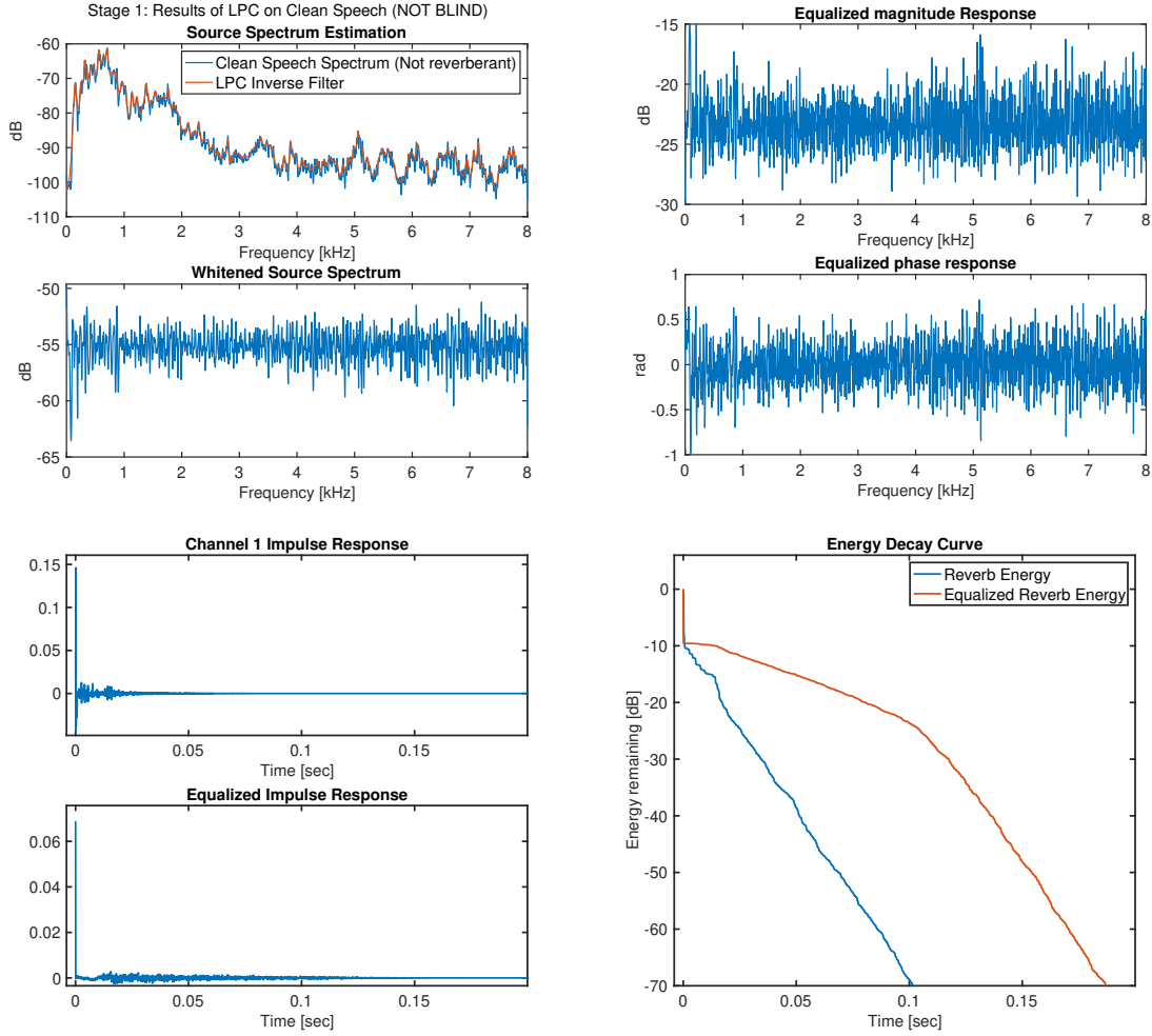
Figure A.5: Delay-and-Predict dereverberation performance with source whitening prediction order p_1 = 200 and multichannel linear prediction order p_2 = N_{60}/(M-1) .
