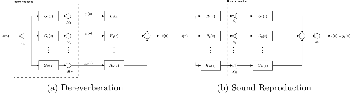
Figure 2.1: Block diagram the formulations of MINT filtering: dereverberation (a) and sound reproduction (b)
