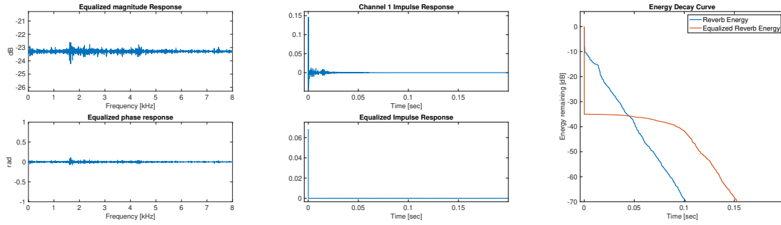
Figure A.3: Delay-and-Predict dereverberation performance with multichannel linear prediction order p_2 = 0.75 \cdot N_{60}/(M - 1) , where N_{60} is the number of samples corresponding to the T60 and M is the number of channels (i.e., suboptimal with respect to the MINT condition based on T60 rather than the FIR RIR length). Figure 3.2 shows the common source whitening filter used.
