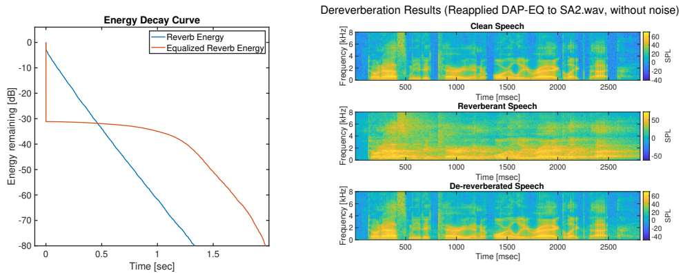
Figure 3.6: DAP Equalizer performance (EDC and Spectrogram) with the source-whitening filter computed using clean speech (i.e., not blind)
