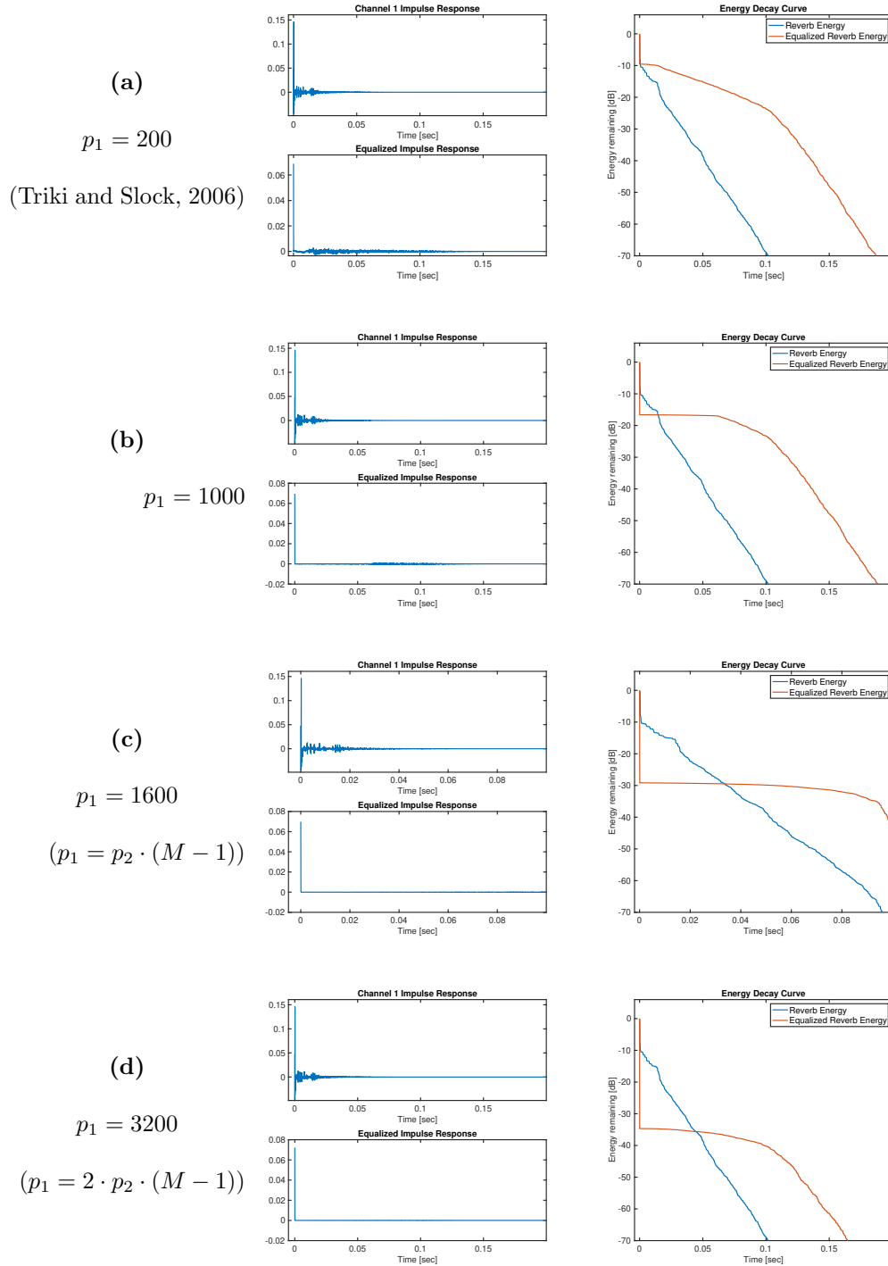
Figure 3.4: Impact of source-whitening prediction order ( p_1 ) on DAP dereverberation performance. Prediction orders are quantified relative to the MC-LP order, which was set to p_2 = N60 / (M - 1)
