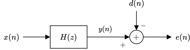
Figure 2.2: Block diagram for supervised optimal filtering, which attempts to produce a desired output, d(n) , from a known input, x(n)
