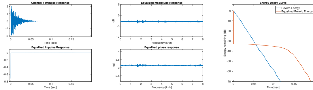
Figure 3.14: DAP dereverberation performance (after linear combiner) with no time delay between channels (i.e., time aligned)
