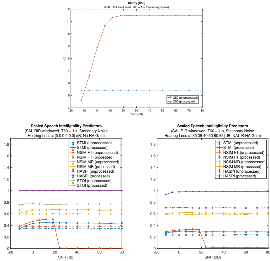
Figure 4.24: Evaluation of delay-and-predict dereverberation performance with autocorrelation regularization in the presence of noise as a function of SNR. RIRs were generated by applying a variable decay-rate exponential window to a measured RIR (The SAL room from the MYRiAD database, T60 = 2.2 s) to set T60 = 1 s. Noise was a multichannel recording of approximately stationary noise (Office ventilation noise from the HRIR database).
