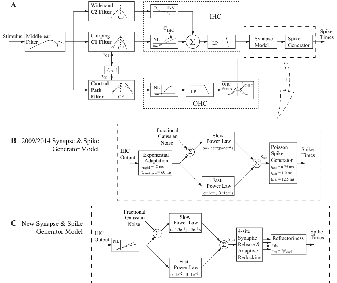
Figure 1.8: Mammalian auditory periphery model used in the NSIM and STMI predictors of speech intelligibility (Bruce et al. , 2018) Used with permission of Elsevier Science, Figure 3 from Bruce et al. (2018) ©2018; permission conveyed through Copyright Clearance Center, Inc.
