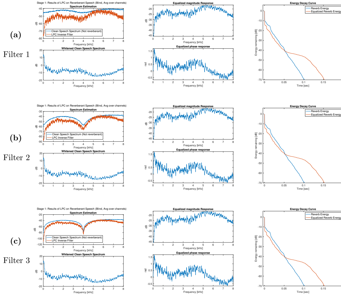
Figure 3.11: Impact of source spectral dynamic range on DAP dereverberation performance. The source signal was generated by filtering 60 m sec of speech with filters of various peakiness. Source whitening prediction order was p_1 = 2 \cdot p_2 \cdot (M - 1) and MC-LP was p_2 = N60/(M - 1) . Source Whitening stage was performed on reverberant speech (i.e., blind estimation).
