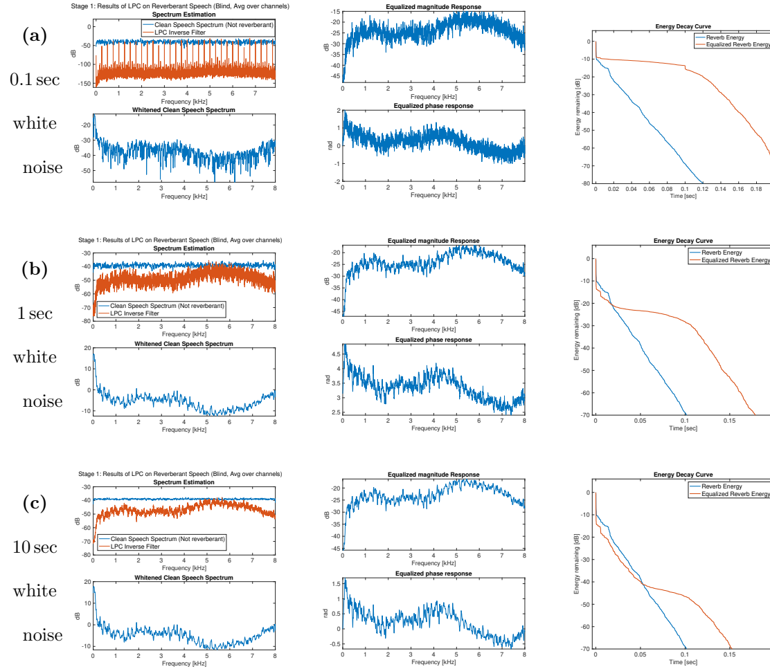
Figure 3.10: Impact of source signal spectrum on DAP dereverberation performance. The source signal in each case was generated by synthetically looping a different length white noise sequence to the same duration of 60 sec (i.e., same data length, different spectra). Source whitening prediction order was p_1 = 2 \cdot p_2 \cdot (M - 1) and MC-LP order was p_2 = N60/(M - 1) . Source Whitening stage was performed on reverberant speech (i.e., blind estimation).
