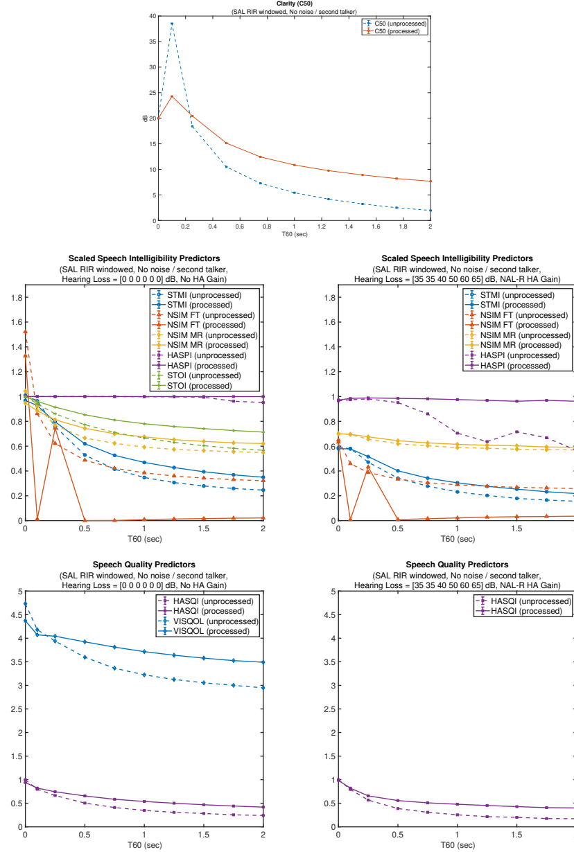
Figure A.12: Evaluation of delay-and-predict dereverberation performance with autocorrelation regularization as a function of T60. Prediction orders were p_2 = 5333 and p_1 = 20000 (i.e., according to T60_{\max} = 1 sec for M = 4 and f_s = 16 kHz).
