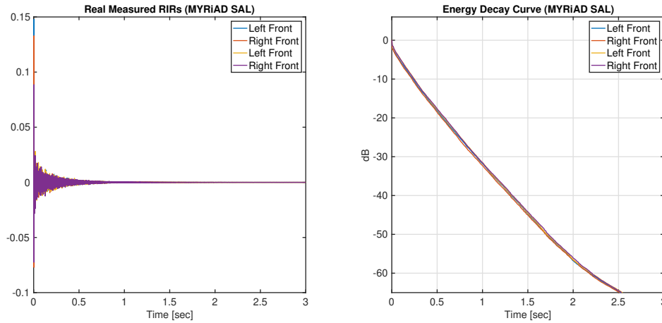
Figure 4.4: EIR and EDC of the MYRiAD database SAL room
