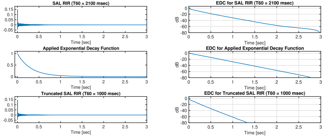
Figure 4.11: Example of how SAL was processed by applying additional exponential decay as a window to manipulate T60 synthetically.
