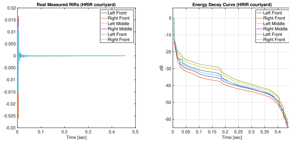
Figure 4.2: EIR and EDC of the HRIR database courtyard room
