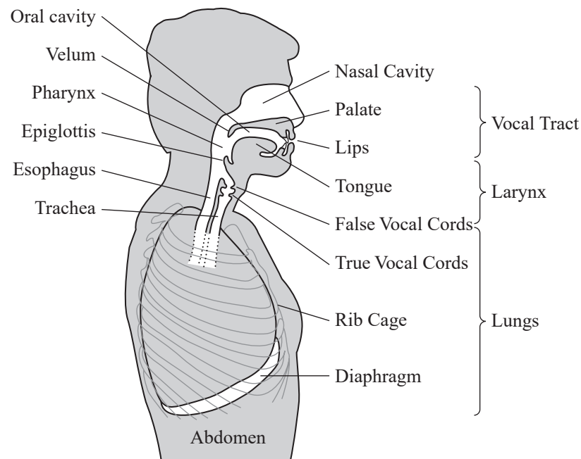
Figure 1.5: Human speech production system. Used with permission of Pearson, Figure 3.2 from Quatieri (2002) ©2002.
