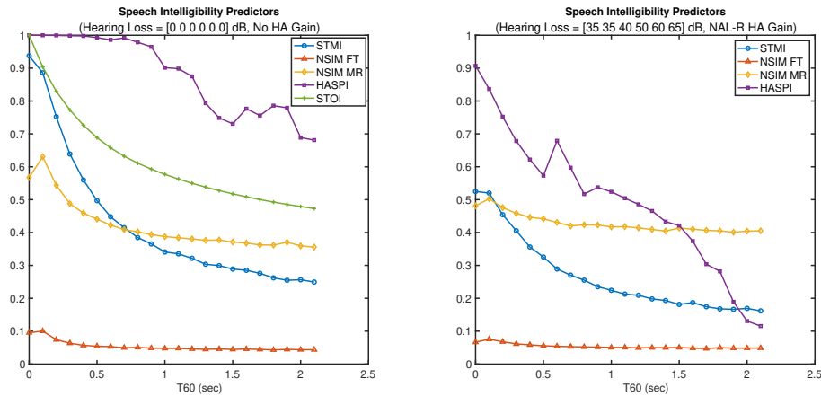
Figure 4.14: Impact of practical reverberation (SAL room from MYRiAD database exponentially windowed to control T60) on SI predictors with and without hearing loss. NAL-R linear hearing aid amplification included in hearing loss case for metrics that including modeling of hearing loss. Scaling applied to NSIM and STMI values to better view all metrics on the same plot. The direct sound / early reflections of SAL RIR were reduced by 6 dB as shown in Figure 4.13.
