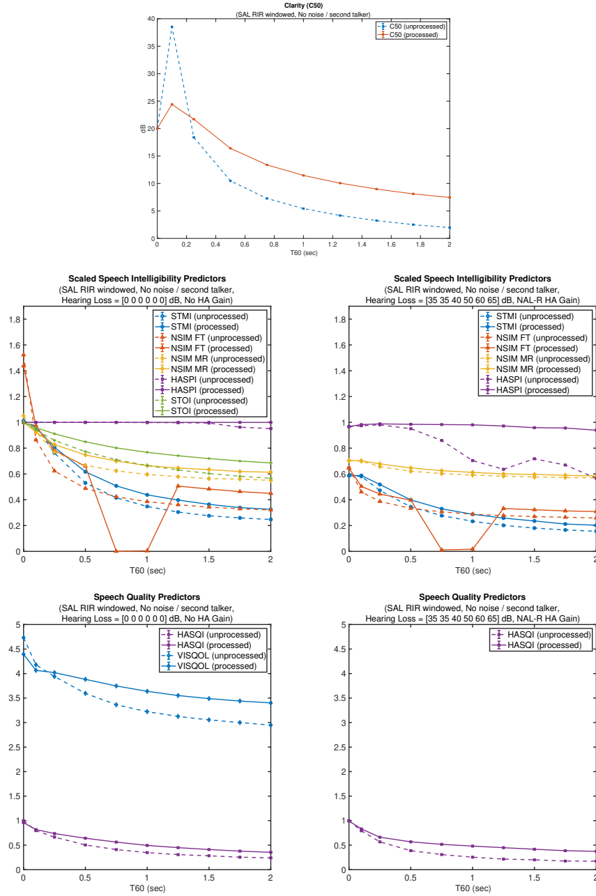
Figure 4.21: Evaluation of delay-and-predict dereverberation performance with auto-correlation regularization as a function of T60. Prediction orders were p_2 = 2667 and p_1 = 10000 (i.e., according to T60_{\max} = 500 msec for M = 4 and f_s = 16 kHz). RIRs were generated by applying a variable decay-rate exponential window to a measured RIR (The SAL room from the MYRiAD database, T60 = 2.2 s) to control T60. No Noise or Interfering talker were included.
