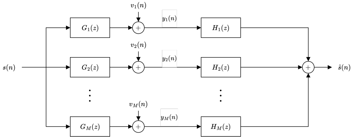
Figure 2.5: Block diagram for multichannel inverse filtering, which attempts to reproduce the known input, s(n) , to an unknown multichannel system \{G_1(z), G_2(z), \dots, G_M(z)\} , by filtering and summing the M microphone signals, \{y_1(n), y_2(n), \dots, y_M(n)\} , with a set of FIR filters, \{H_1(z), H_2(z), \dots, H_M(z)\}
