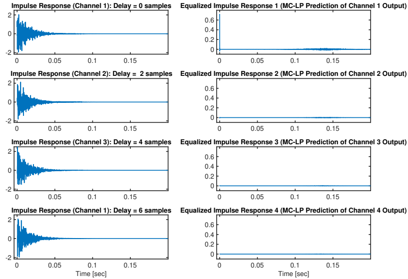
Figure 3.13: Vector-valued EIR performance prior to linear combiner with an incremental 2-sample delay added to each channel (i.e., not time aligned).
