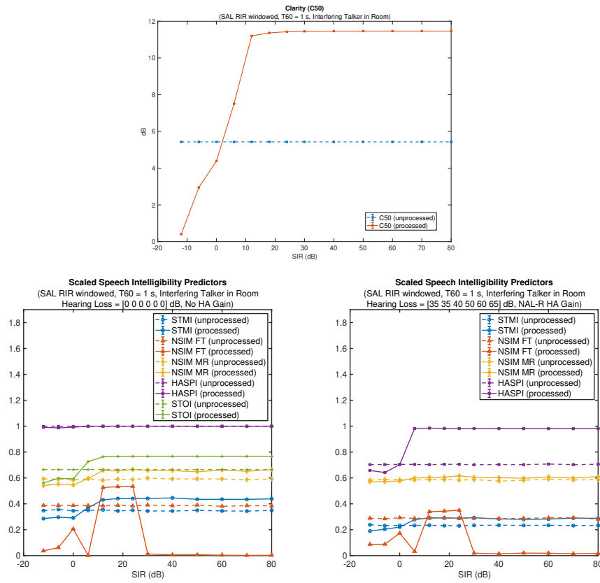
Figure 4.26: Evaluation of delay-and-predict dereverberation performance with auto-correlation regularization in the presence of a non-co-located secondary talker in the same room as a function of signal-to-interference ratio (SIR). RIRs were generated by applying a variable decay-rate exponential window to a measured RIR (The SAL room from the MYRiAD database, T_{60} = 2.2 s) to set T_{60} = 1 s.
