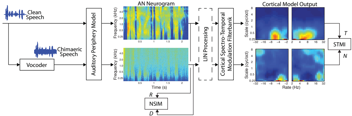
Figure 1.9: Schematic for generation of NSIM and STMI predictors of speech intelligibility. Note that the usage of Chimaeric speech as the test signal in this depiction is specific to the study being conducted by (Wirtzfeld et al. , 2017). Reproduced with permission from Springer Nature, Figure 2 from Wirtzfeld et al. (2017) ©2017; permission conveyed through Copyright Clearance Center, Inc.
