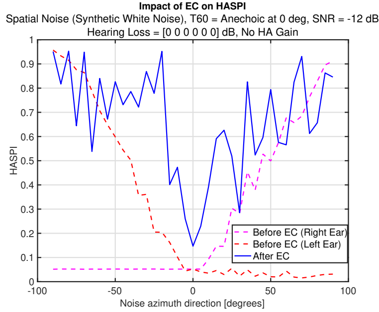
Figure A.9: Impact of EC algorithm on speech intelligibility (using HASPI) as a function of noise direction, anechoic directional speech and noise.
