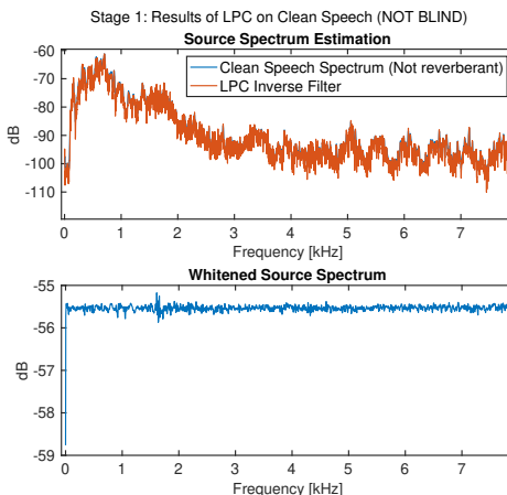
Figure 3.2: Source whitening results using a p_1 = 4000 order linear predictor. The prediction error filter coefficients were computed based on clean speech and the same filter was used in all tests in this section to assess the MC-LP stage of the DAP algorithm in isolation.
