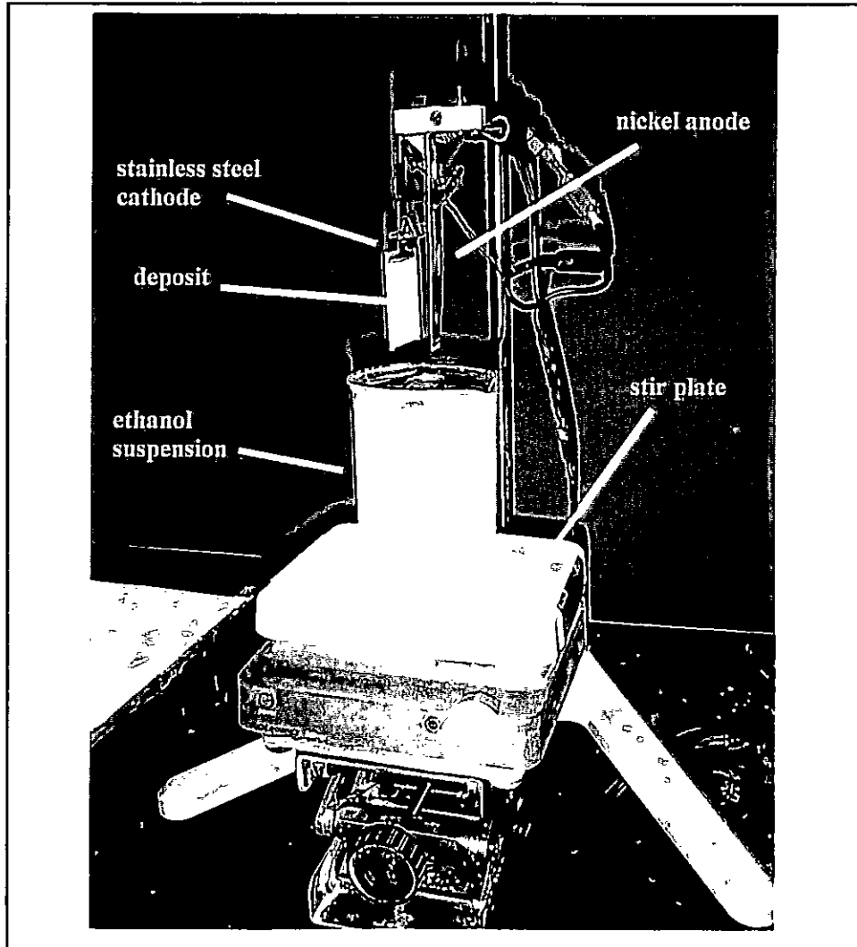
Figure 3.1 Experimental setup for electrophoretic deposition (EPD).
