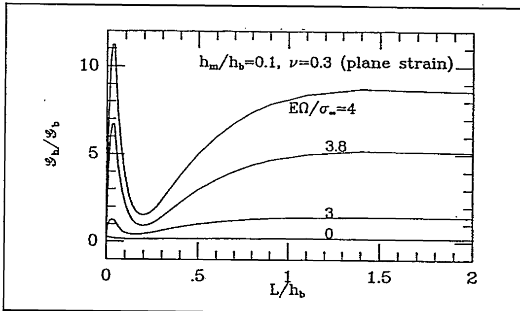
Figure 2.28 Energy release rate ratios calculated for branch cracks as a function of (normalized) crack length (Lu, 1996).
