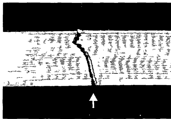
Figure 4.9 (n) Composite C13
