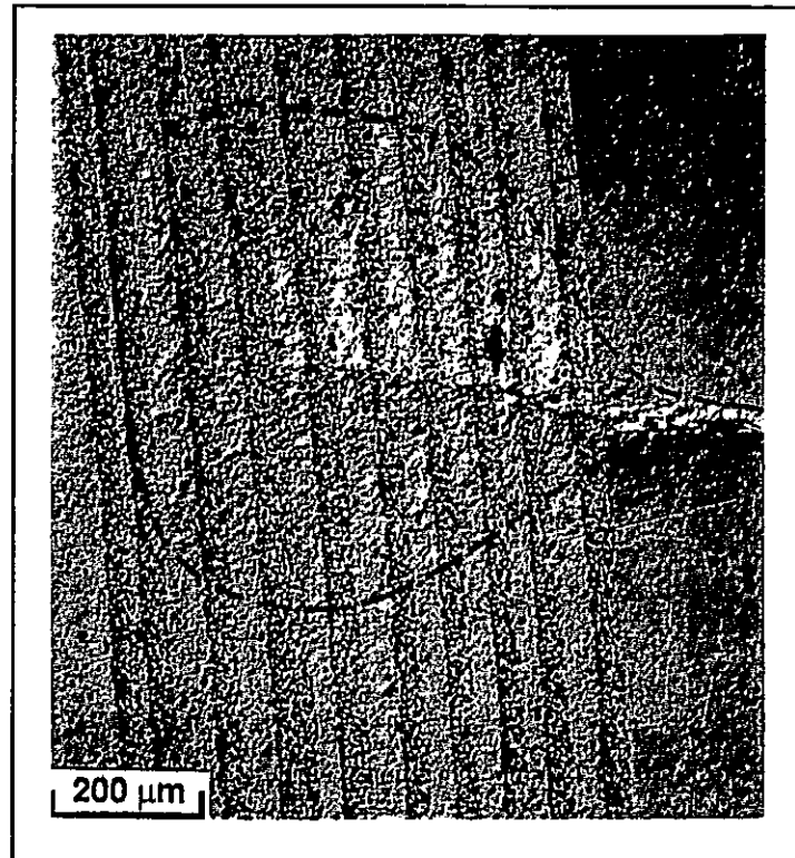
Figure 2.29 The widening of the transformation zone ahead of a crack propagating through a series of \text{Al}_2\text{O}_3+\text{ZrO}_2 layers (Marshall et al. , 1991).
