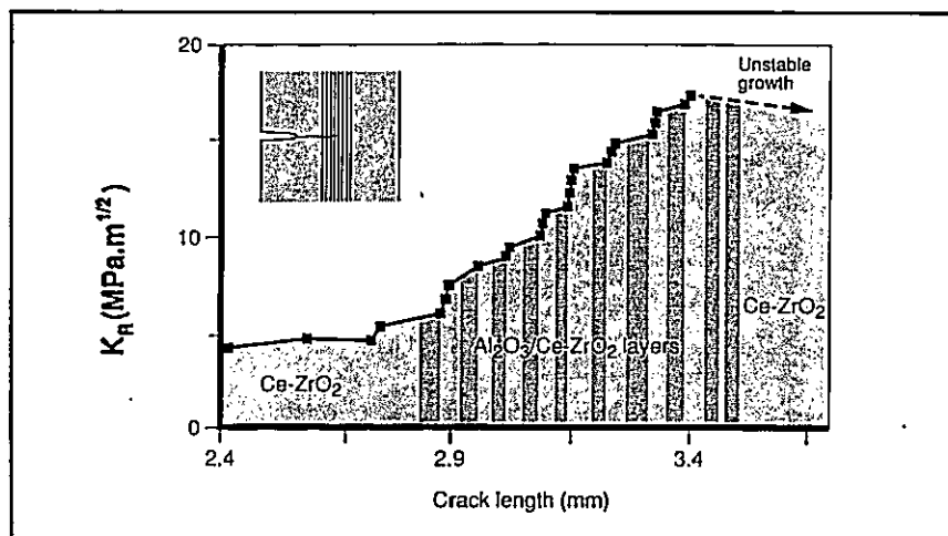
Figure 2.30 R-curve (T-curve) measurements for a crack propagating through a series of \text{Al}_2\text{O}_3+\text{ZrO}_2 layers (Marshall et al. , 1991).
