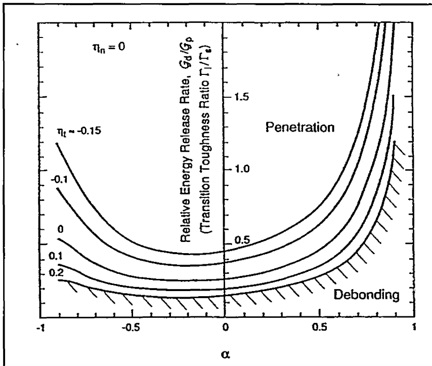
Figure 2.26 The energy release ratio as a function of \alpha for various values of \eta_t (He et al. , 1994).
