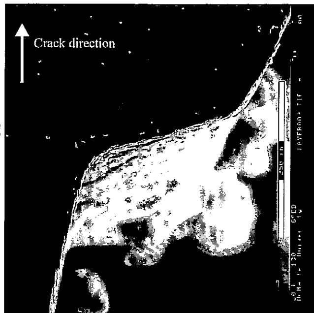
Figure 4.14 (a,b) ESEM micrographs of the deflection steps in the path of an unstable crack.
