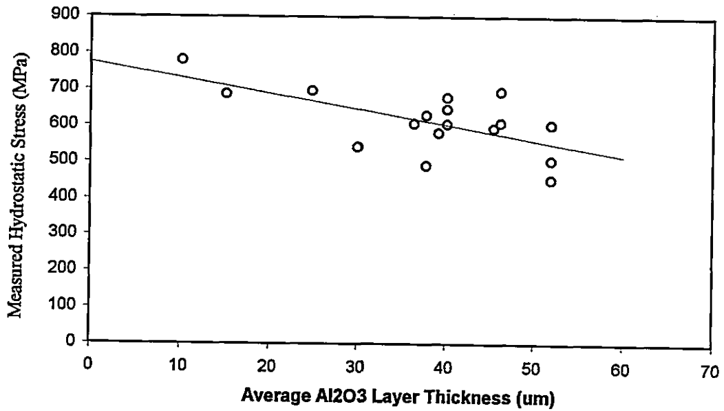
Figure 4.7(a) Compressive hydrostatic stress for composites < 10 Al 2 O 3 Vol% as a function of the average Al 2 O 3 layer thickness.
