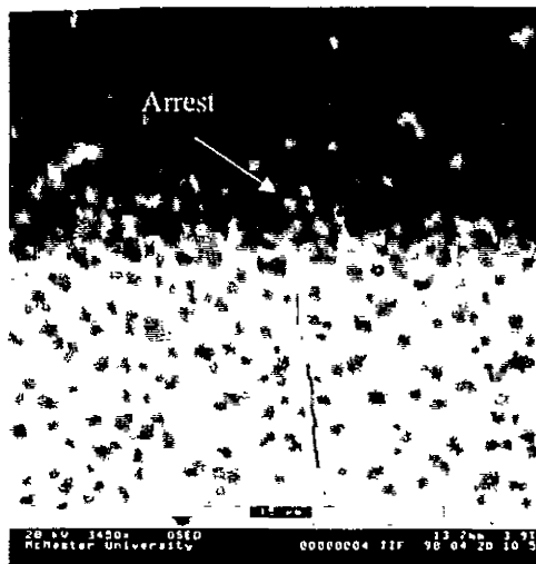
(d) Closer examination of the crack tip indicates it has arrested at the TZ3Y/ \text{Al}_2\text{O}_3 interface.
