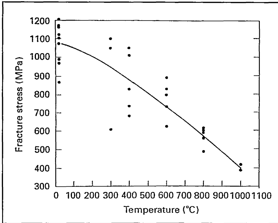
Figure 2.11 4-point bend strength of Y-TZP (at 0.5 mm min -1 ) as a function of temperature (Govilla, 1995).
