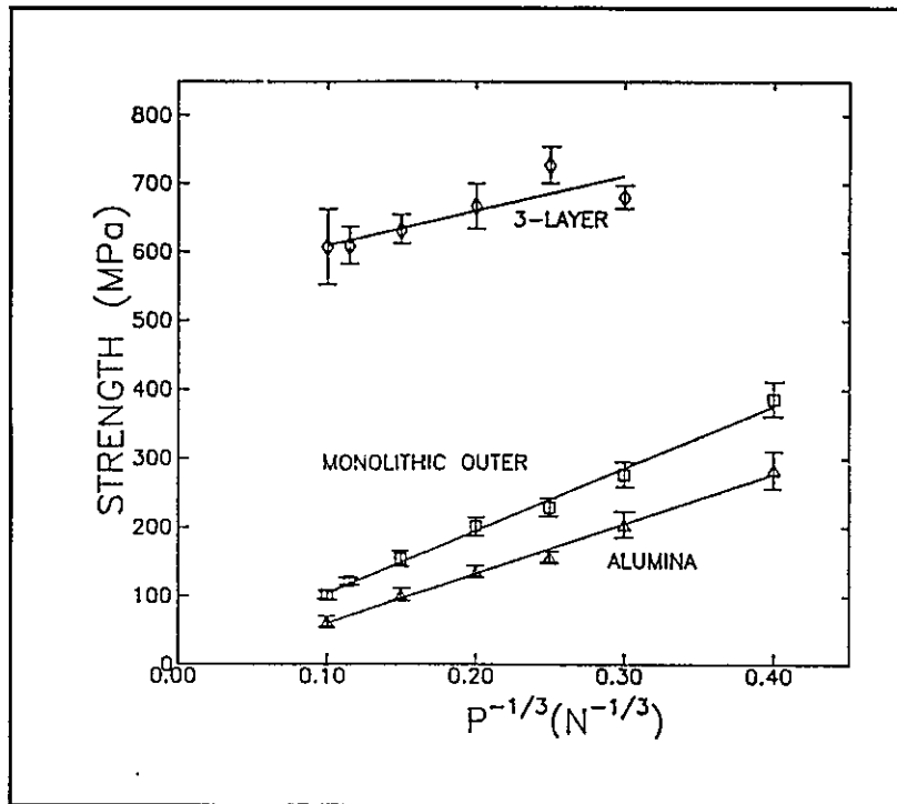
Figure 2.33 Indentation-strength results for the layered composite, monolithic \text{Al}_2\text{O}_3+15\text{vol}\% \text{ZrO}_2 (tetragonal) and monolithic \text{Al}_2\text{O}_3 (Hansen et al. , 1988).
