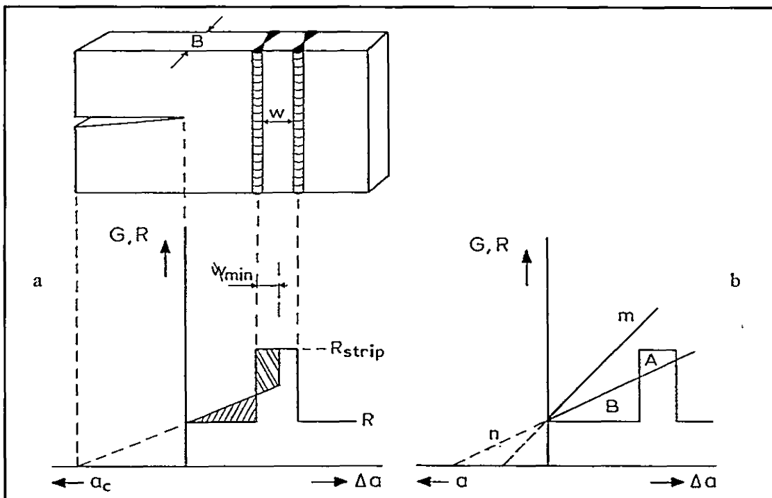
Figure 2.6 Layer of high toughness welded in a metal plate for crack arrest (Bluhm, 1969).
