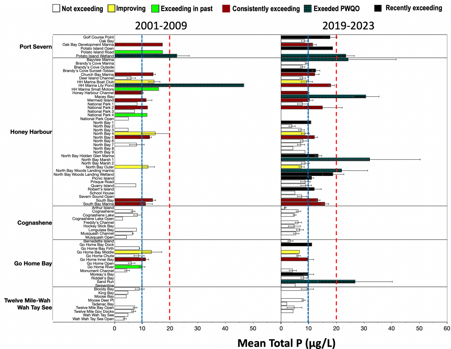
Figure 7: Comparison of mean TP (µg/L) in Period 2 relative to Period 1. Exceedances are with respect to the GBWQO (< 10 µg/L; blue short-dashed line) and the PWQO (< 20 µg/L; red long-dashed line).
