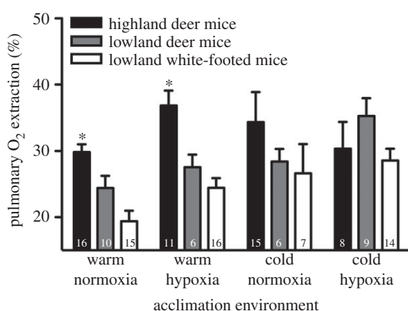
Figure 3. Pulmonary O_2 extraction at \dot{V}_{O_{2max}} was found to vary across populations and acclimation treatments. See figure 1 for symbol definitions and statistical details.
