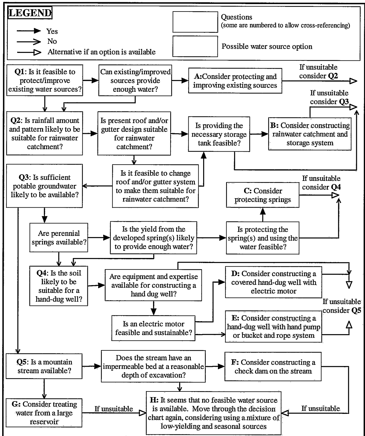
Figure 8: Decision tree for choosing potential water sources
