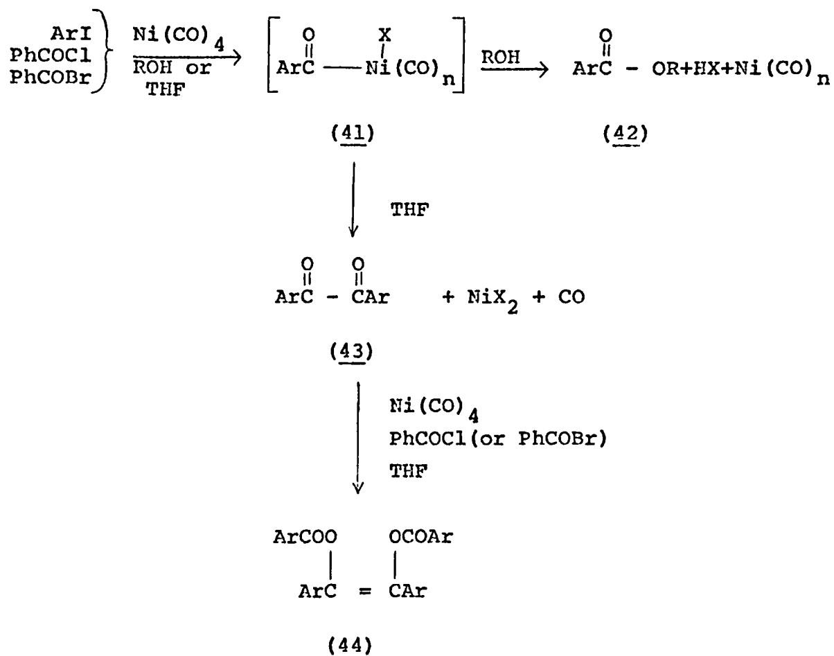
Fig. 3. Reactions of nickel carbonyl with some organic halides
