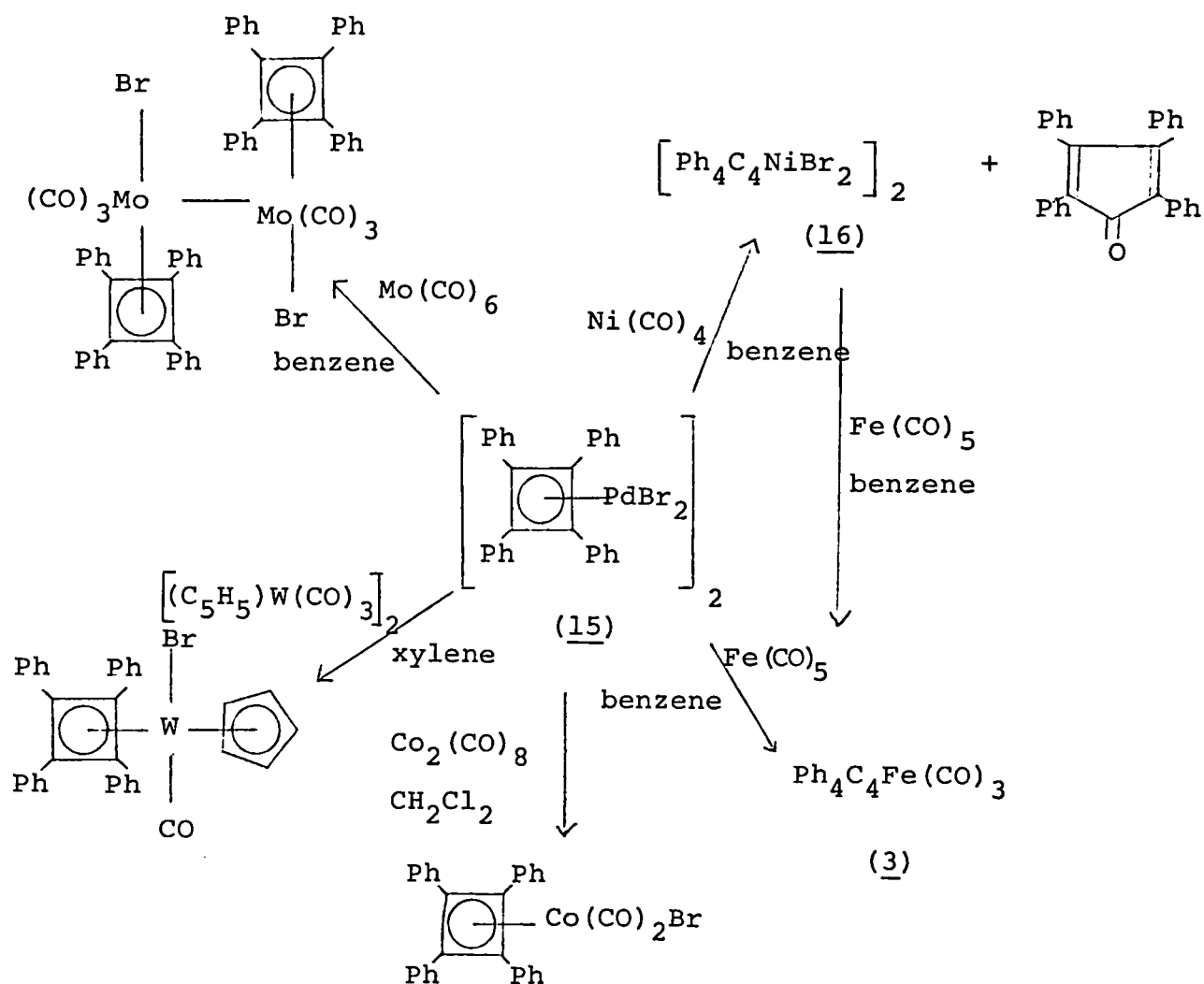
Fig. 2. Synthesis of cyclobutadiene-metal complexes by ligand-transfer reactions.
