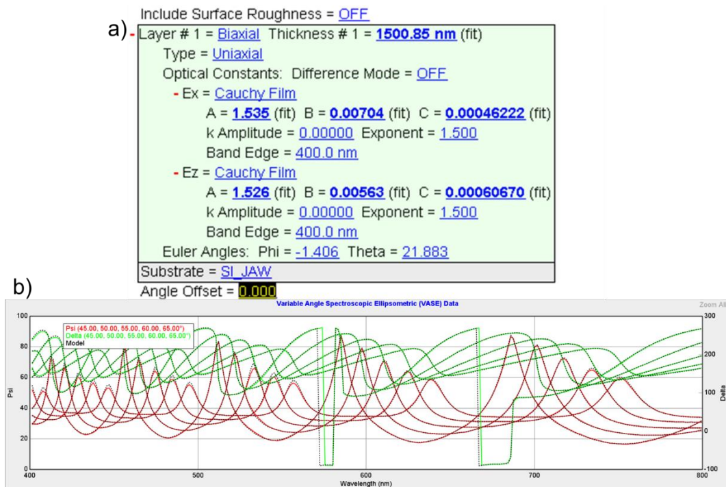
Figure 9.1: Nominal parameters for modeling BCB thickness in VASE. a) parameters for the biaxial Cauchy film and b) Psi and Delta for a thick (1.5 \mu\text{m} ) BCB layer in the 400 – 800 nm wavelength range.
