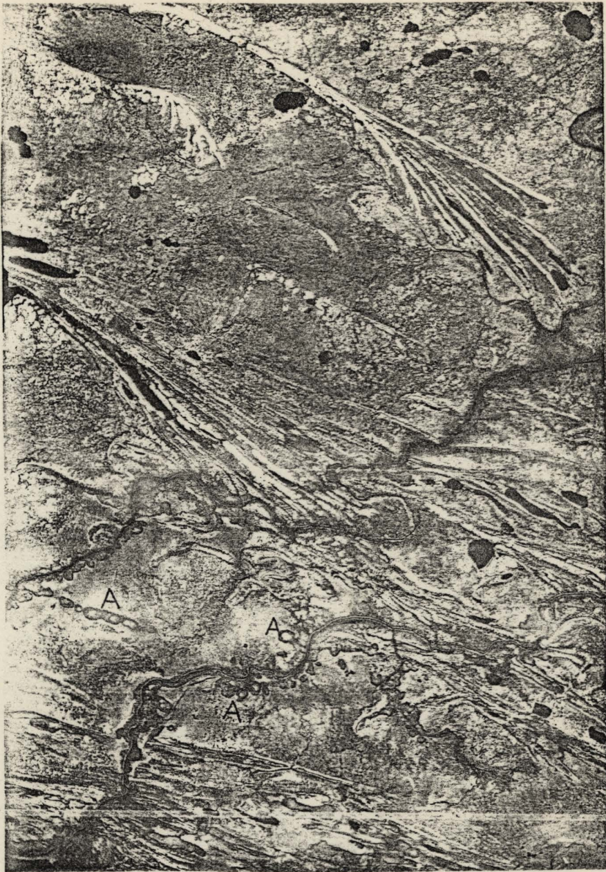
Figure 3.5 Collapse scars located in central parts of peat plateaus (A)
