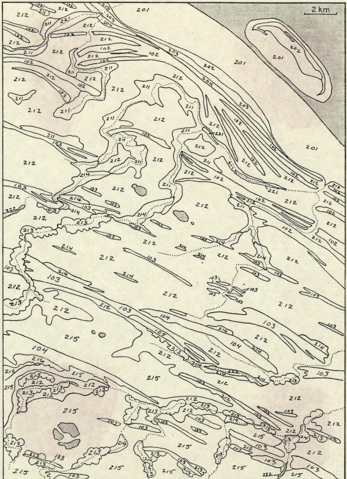
Figure 4.7 Spatial model of landscape at Pen Island. For identification of classes, see Table 4.II.
