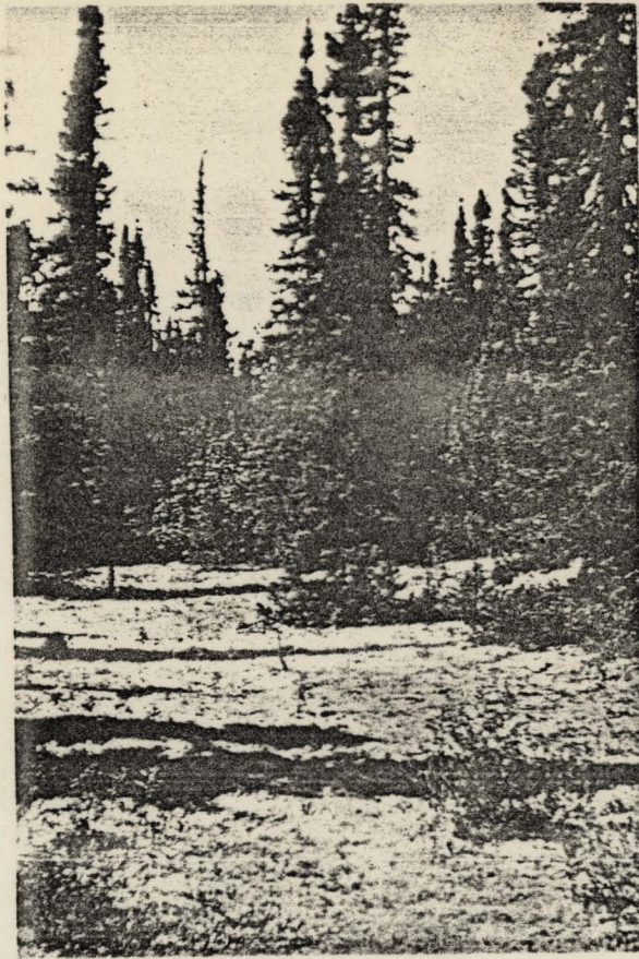
Figure 3.19(a) Spruce-lichen woodland (Site 11)
