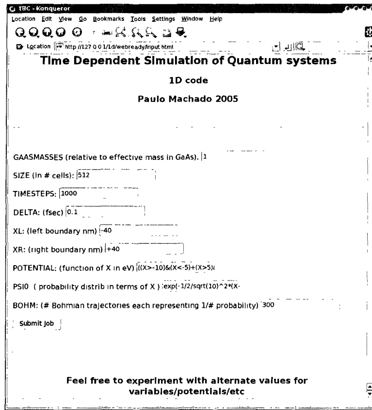
Figure 3.6: Typical run of the code via web interface
