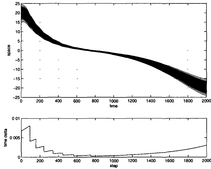
Figure 4.22: Dynamic timescale, abrupt declines represent time step adjustments caused by error conditions
