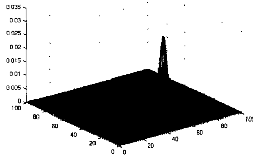
Figure 6.1: Initial wavepacket ( t=0 )
