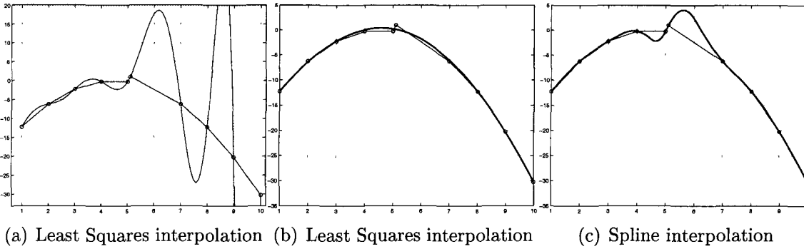
Figure 4.9: Interpolation methods compared
