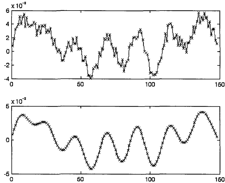
Figure 4.7: The residue of a particular wavefunction and the result of low pass filtering instance in a least squares way. Once that is determined, the residue \text{Res}(x) = C(x) - \text{Poly}_m(x) is calculated and can be expanded in a (discrete) sine series (DST) as in equation 4.1.
