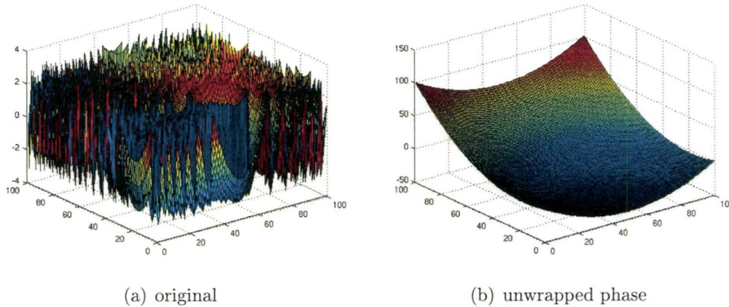
Figure 6.7: A practical case of the phase problem and its solution
