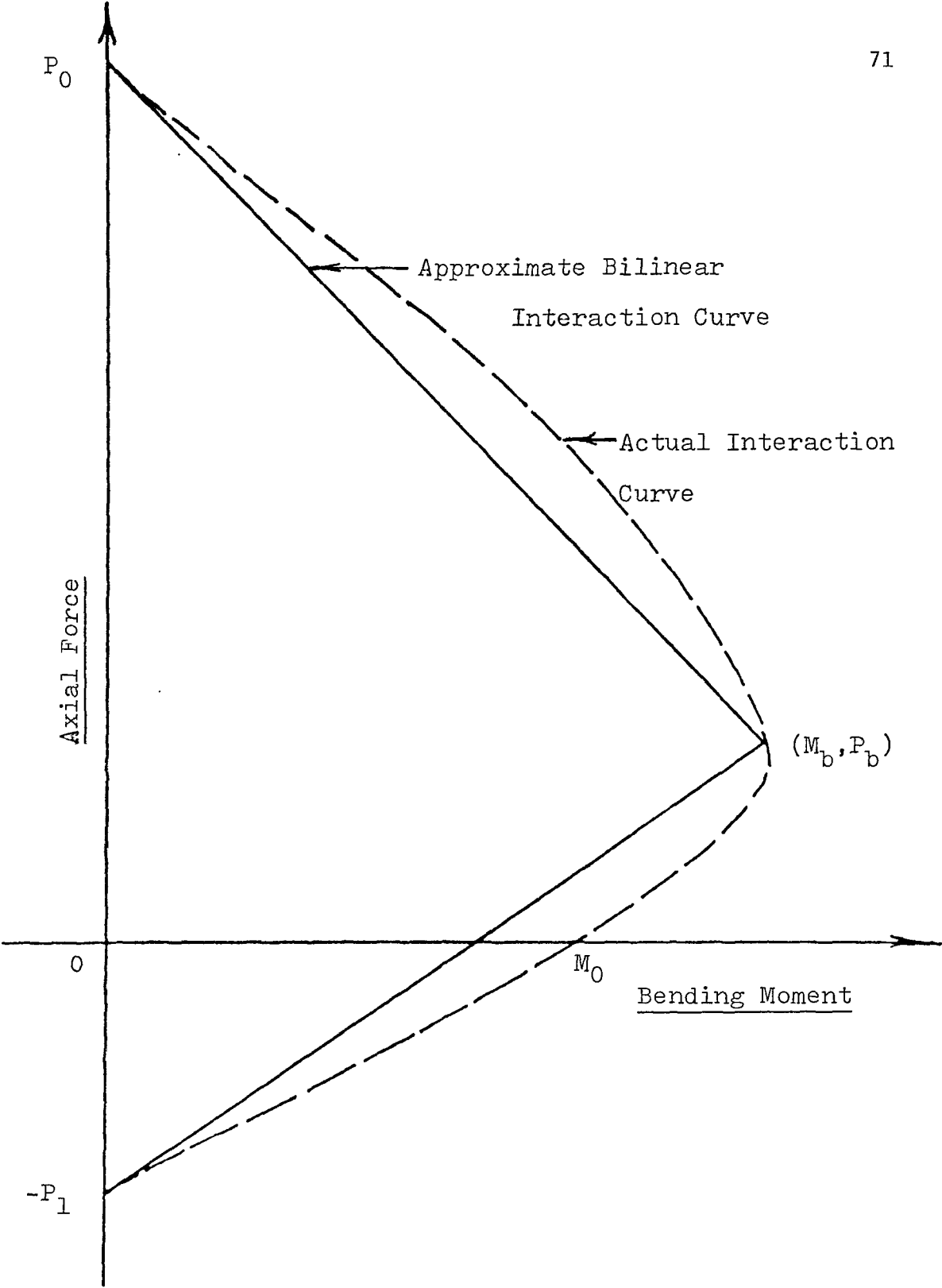
FIGURE 3-2 INTERACTION CURVE
