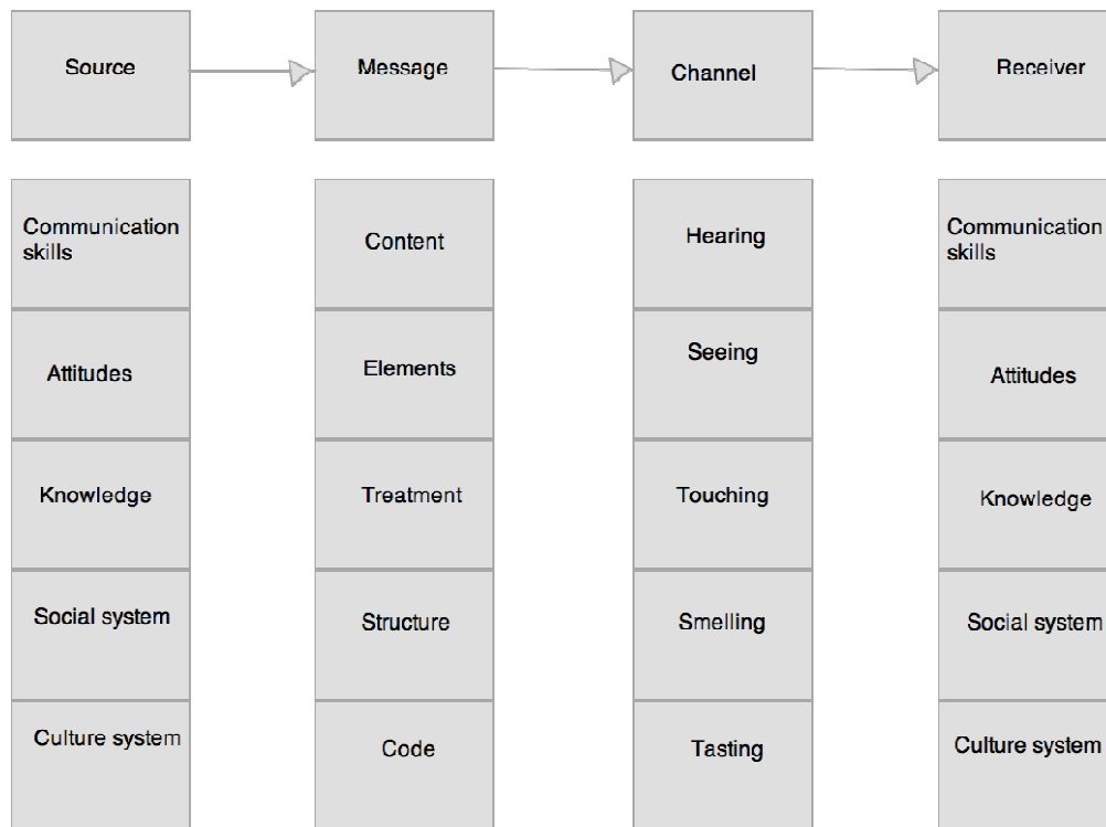
Figure 7: Berlo's Communication Process Model
