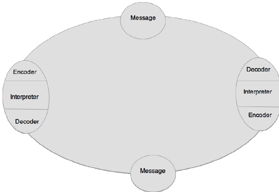
Figure 6: Circular Model of Communication
