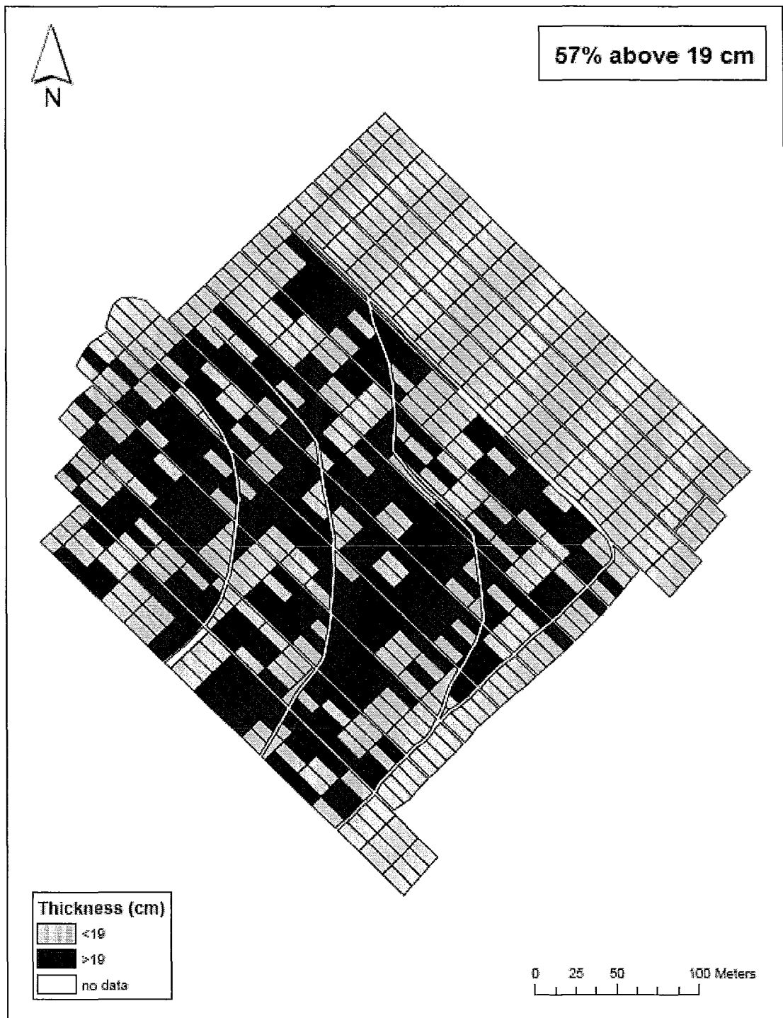
Figure 4.13: Locations estimated to be at or above the 19 cm threshold 17 years post-restoration at Bois-des-Bel.
