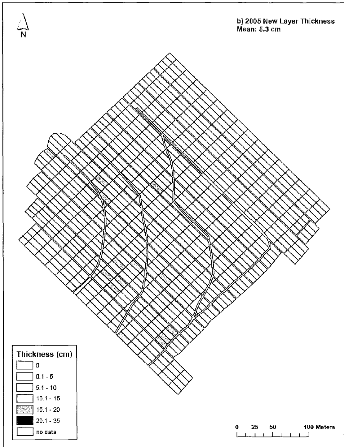
Figure 4.2: Thickness of the new peat layer at the restored and cutover portions of Bois-des-Bel in 2005 (6 years post-restoration).
