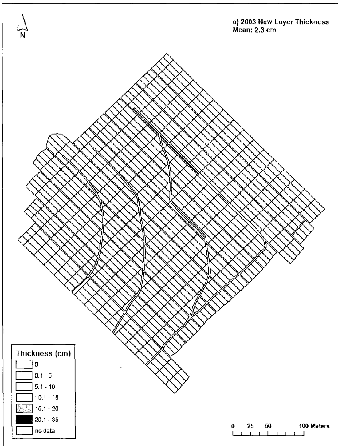
Figure 4.1: Thickness of the new peat layer at the restored and cutover portions of Bois-des-Bel in 2003 (4 years post-restoration).
